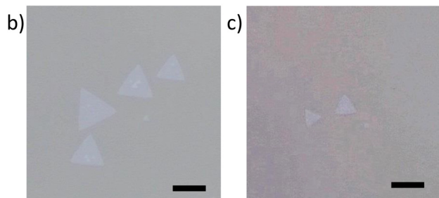
Fig. 1 H 2 -annealing of sapphire. (a) Diffraction pattern of H 2 -annealed sapphire measured by LEED at 63 eV, showing the (\sqrt{31} \times \sqrt{31})R \pm 9^\circ surface reconstruction. (b) WS 2 crystals grown on H 2 -annealed sapphire. (c) WS 2 grown on standard sapphire. The scale bars are 20 \mu\text{m} .
