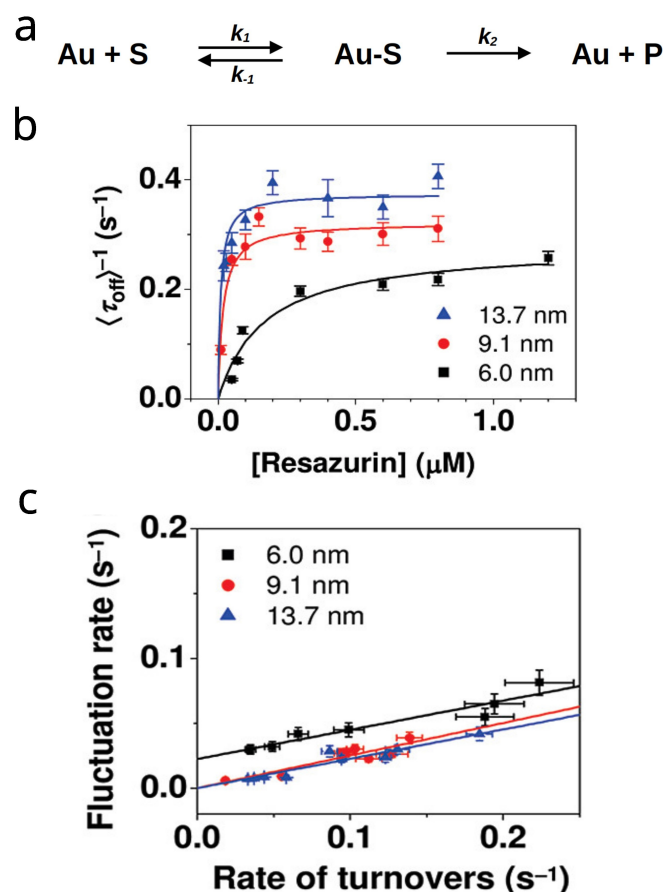
Fig. 2 (a) Michaelis-Menten chemical reaction for nanocatalysis. (b) mean turnover rate as a function of substrate concentration for Au-nanoparticle of different size (c) Activity fluctuation rate in the turnovers from the Au-nanocatalyst. Figures (b,c) reproduced with permission from ref 14 . Copyright 2009 American Chemical Society.
