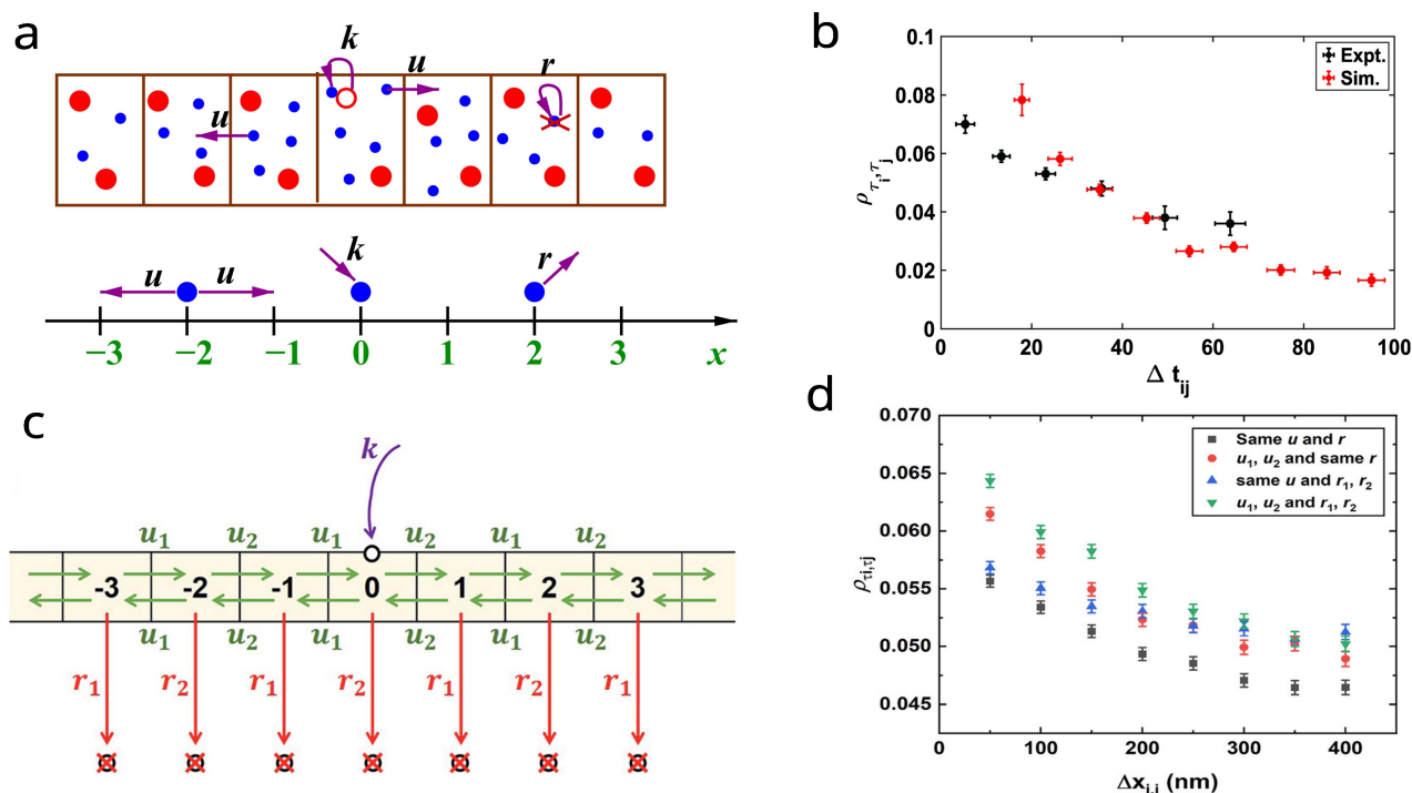
Fig. 7 Communication in the nanoparticle catalysis (a) the schematic diagram of hole creation, migration, and disappearance on a nanorod is divided into segments of equal length. The panel at the bottom shows the discrete state model, where the lattice sites are labeled as integers for different segments. (b) Experimental and theoretical (simulated) Pearson's cross-correlation coefficients against average time separation \Delta t_{ij} of subsequent reactions at segments i and j on the Pd nanorod. (c) Model for catalytic communication with heterogeneous rate constants. (d) Pearson's cross-correlation coefficients varied with average separation \Delta x_{ij} for two segments i and j on the nanorod and comparison between heterogeneous and homogeneous cases. Figures (a, b) reproduced from ref 158 published by PNAS under CC BY-NC-ND 4.0. Figures (c,d) reproduced with permission from ref 143 . Copyright 2023 American Chemical Society.
