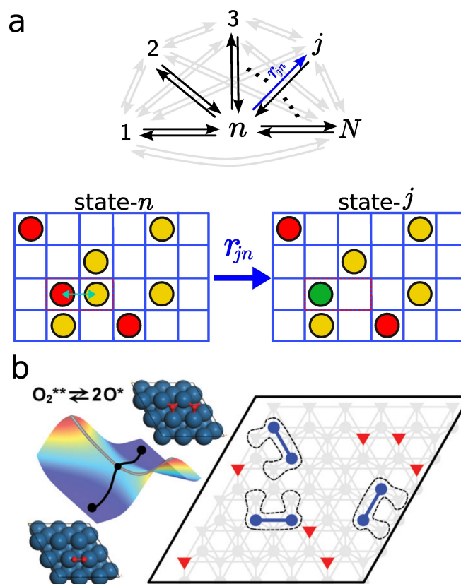
Fig. 1 (a) Schematic diagram for a network of N discrete states. A discrete state is a coarse grained version of long lived catalytic state where each discrete state can be a specific configuration of microstates of the catalyst. (b) Schematic for O_2 dissociation on a catalytic surface where different orientations of the adsorption can also represent different discrete states. Panel (b) is reproduced with permission from Ref 82 , Copyright 2012 American Chemical Society.
