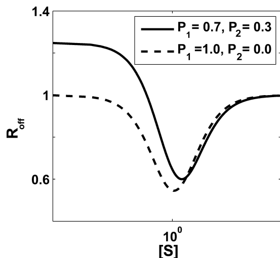
Fig. 4 Randomness parameter for two site heterogeneous enzyme as a function of substrate S concentration. Dotted line is for turnover from a single reaction and solid line is for the turnover from two different reaction. P_1 and P_2 denote the fractional contribution of each reaction in the turnover. Reproduced from ref 144 , Copyright (2015), with permission from Elsevier.
