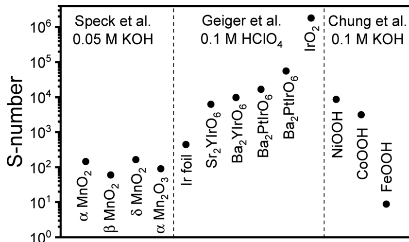
Fig. 6 Summary of S -numbers determined for \text{MnO}_x catalysts obtained by Speck et al. 96 in alkaline media, for \text{IrO}_x catalysts in acidic media determined by Geiger et al. , 145 and for electrodeposited Ni, Co, and Fe oxides determined by Chung et al. 143
