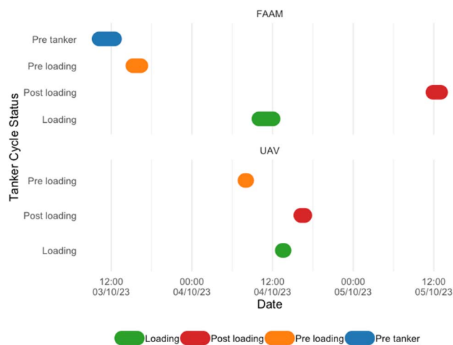
Fig. 2 Dates and details of FAAM and UAV flights and determined part of the oil offloading cycle.
