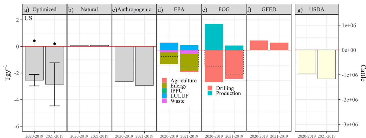
Fig. 1 Differences in 2020–2019 and 2021–2019 \text{CH}_4 emissions over the U.S. from the inversion for (a) net emissions, (b) the natural component, (c) the anthropogenic component, (d) from the U.S. EPA inventory, 19 (e) from the FOG oil and gas inventory, 21 and (f) global fire emissions database. 43 Error bars in panel (a) represent 1-sigma of the anomalies. Panel (g) shows the total number of cattle (heads) in the U.S. 41 EPA and FOG columns show the net results in dashed lines. The points represent the average anomaly for the priors.
