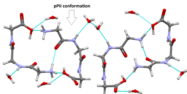
Fig. 1 Hydration-stabilised extended pPII conformation in triglycine (GGG·2H 2 O). The structure highlights the water-mediated hydrogen-bond network stabilising the extended peptide backbone. Crystal structure data were obtained from the Cambridge Structural Database (CSD, refcode ZZZPTQ01).
