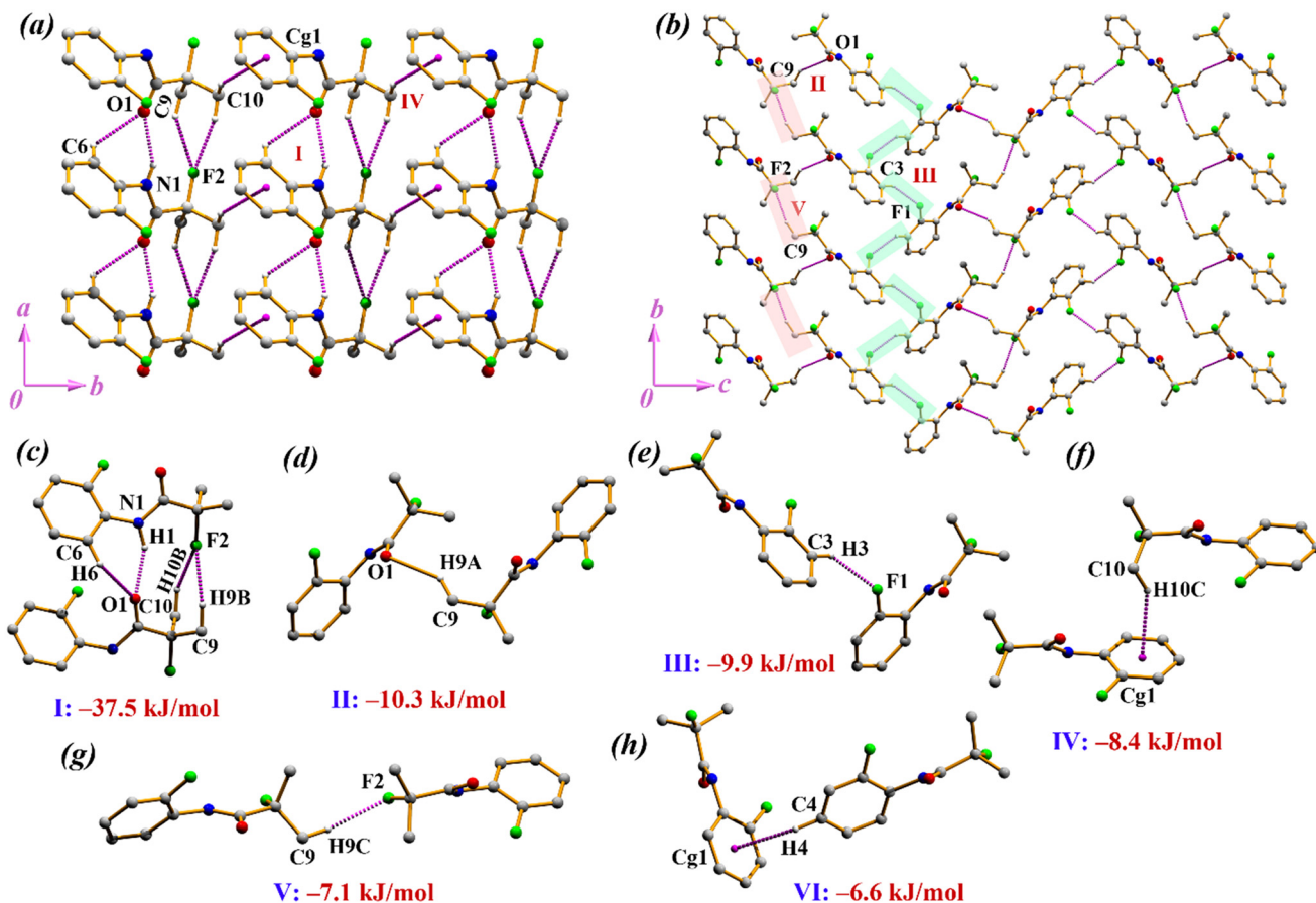
Fig. 2 (a and b) Crystal packing of 1. (c–h) Molecular pairs extracted from PIXEL calculation along with their interaction energies in 1.
