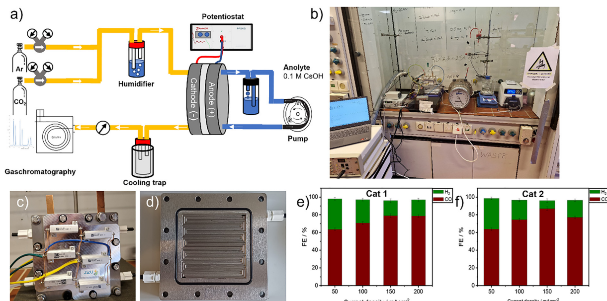
Fig. 5 (a)–(d) Schematic illustration and photograph of a laboratory-scale zero-gap electrolyzer. (e) The \text{CO}_2 reduction performance of ( Cat 1 , Cl-B-SubPc)/CB (800 °C) at 50, 100, 150, and 200 \text{mA cm}^{-2} at 60 °C after two hours of electrolysis. All investigated GDEs possessed a catalytic loading of 0.5 \text{ mg cm}^{-2} of active material. (f) The \text{CO}_2 reduction performance of ( Cat 2 , Cl-B-SubPc)/CB (1000 °C at 50, 100, 150, and 200 \text{mA cm}^{-2} at 60 °C) after two hours of electrolysis. All GDEs examined contained a catalytic loading of 0.5 \text{ mg cm}^{-2} of active material.
