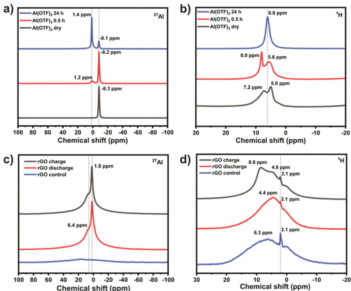
Fig. 4 SS MAS (Solid State Magic Angle Spinning) NMR spectra of \text{Al(OTF)}_3 salt, freeze dried and the cycled rGO cathodes. (a) ^{27}\text{Al} SS MAS NMR spectra of the \text{Al(OTF)}_3 salt. (b) ^1\text{H} NMR spectra of the \text{Al(OTF)}_3 salt. (c) ^{27}\text{Al} SS MAS NMR spectra of the rGO at each condition. (d) ^1\text{H} NMR spectra of the rGO at each condition.
