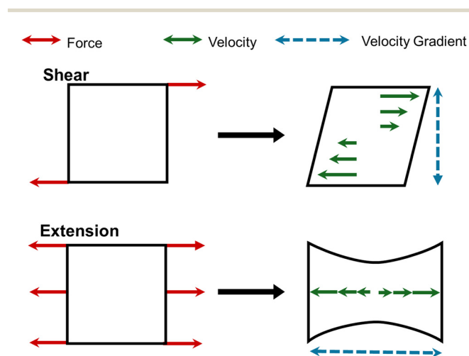
Fig. 3 Illustration of shear and extensional flows.
