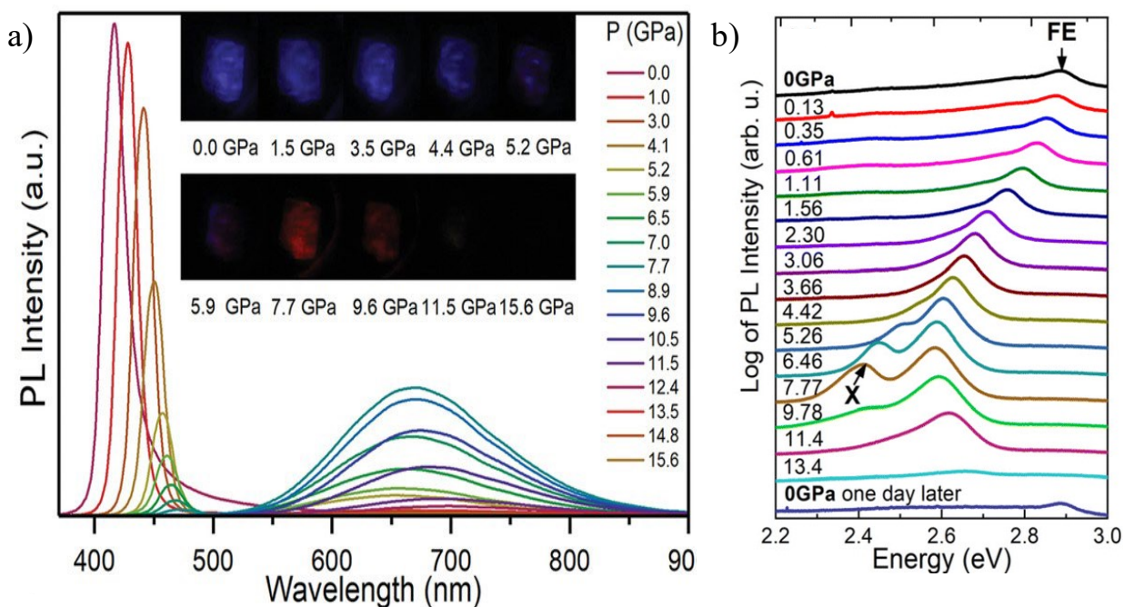
Figure 14. Pressure-induced change in PL nature of RP-type 2D HOIPs. (a) In situ PL spectra upon compression to 15.6 GPa of (\text{PEA})_2\text{PbBr}_4 [52] and (b) In situ PL spectra upon compression to 13.4 GPa of \text{Tz}_2\text{PbBr}_4 [56].
