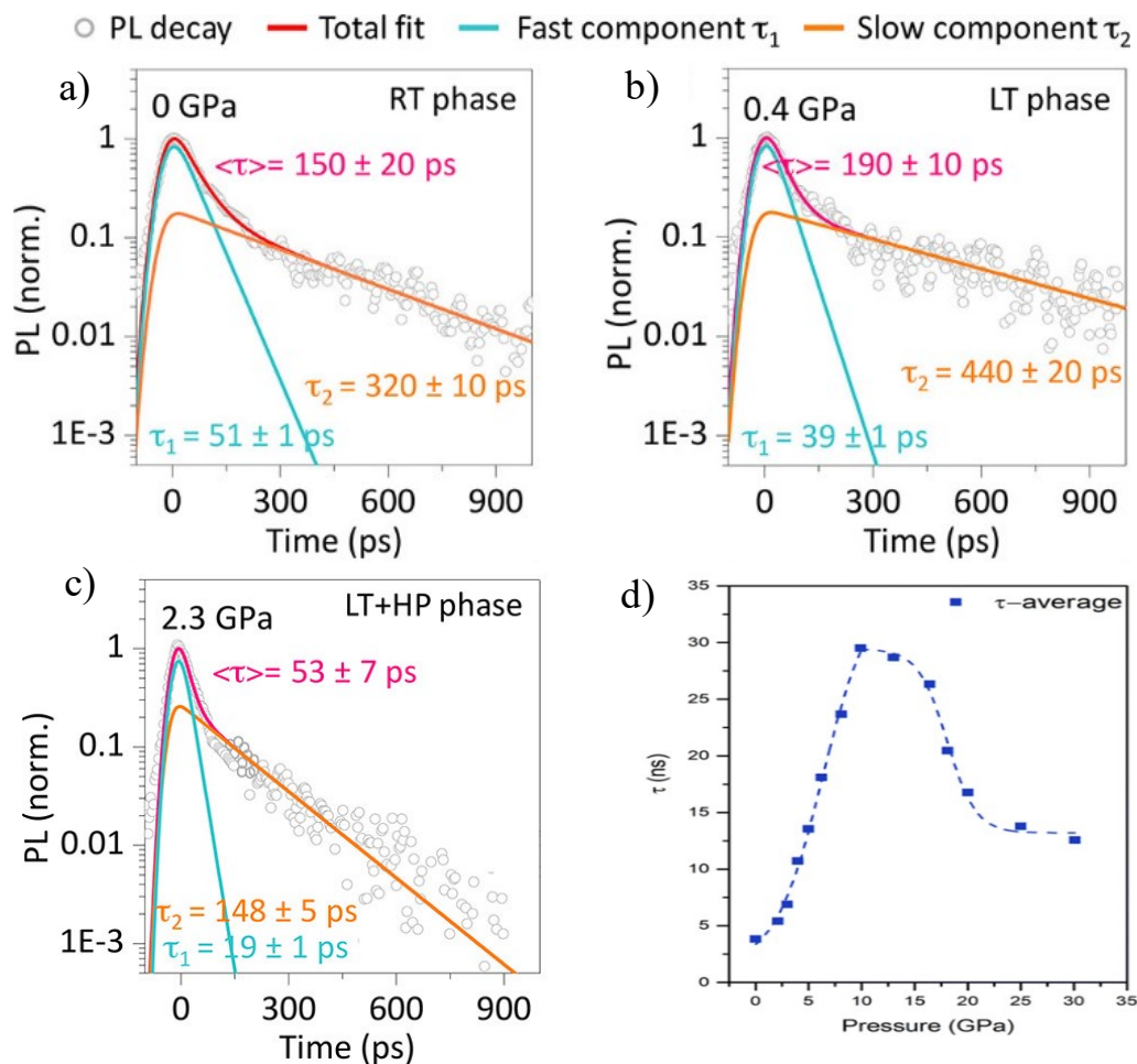
Figure 15. Pressure-induced charge carrier lifetimes of 2D HOIPs. (a), (b), and (c) TRPL spectra of (\text{BA})_2\text{PbI}_4 at 0, 0.4, and 2.3 GPa, respectively [21]. (d) Average PL lifetime as a function of pressure of (2\text{meptH}_2)\text{PbCl}_4 [34].
