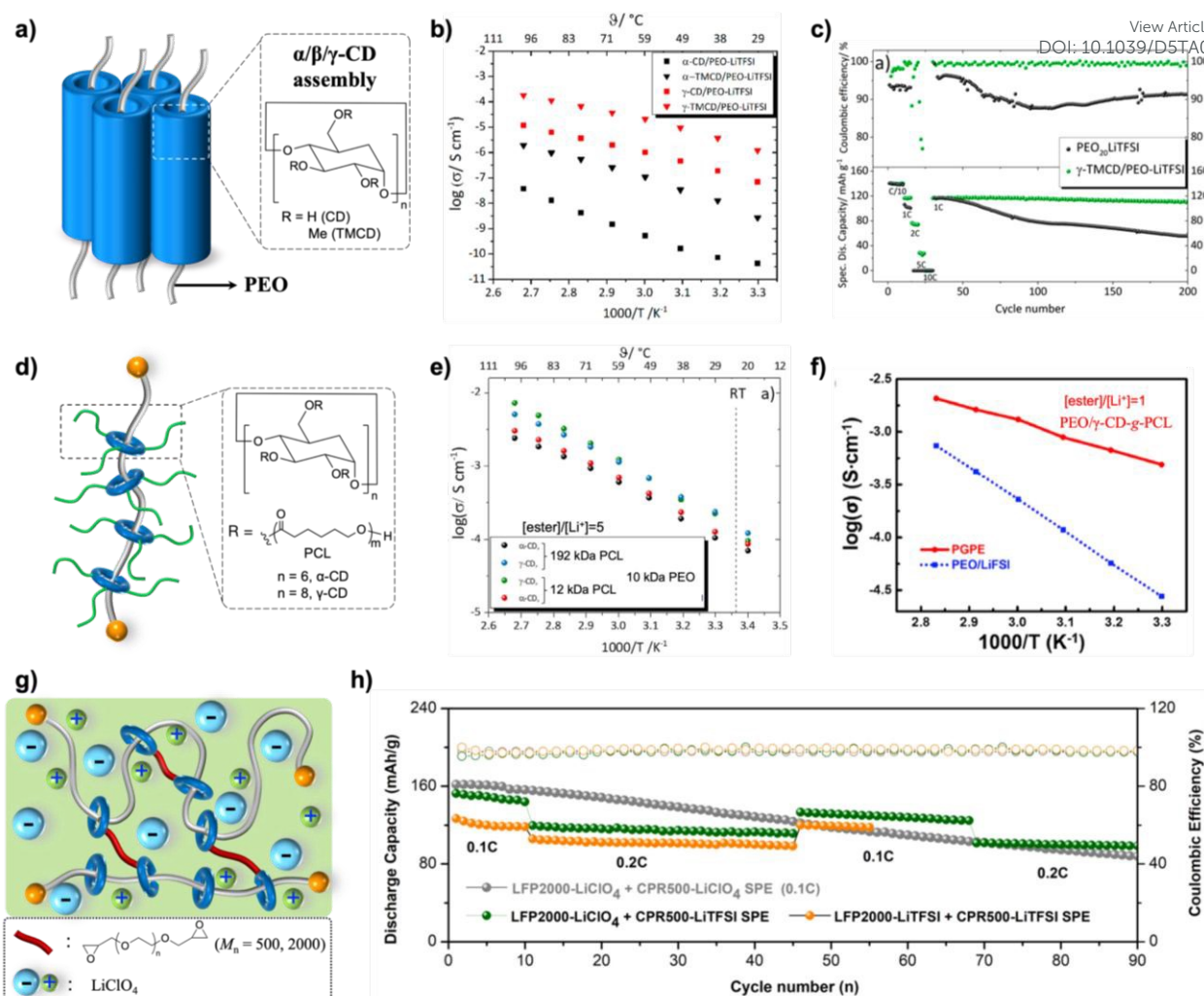
Figure 6 a) Pseudo-PR electrolytes consisting of different CDs and LiTFSI salt show nanochannel structures, and their corresponding temperature-dependent ionic conductivity properties are shown in b). c) The use of a pseudo-PR electrolyte comprising of methylated \gamma -CD and PEO presents improved cycling stability compared with a conventional PEO/LiTFSI electrolyte. d) Schematic PR electrolytes containing PCL-grafted CD wheels. e) The length effect of grafted PCL (12 or 192 kDa) and CD species ( \alpha - or \gamma -CD) on the PR electrolyte ionic conductivities. f) Ionic conductivity of a “polymer-in-salt” electrolyte containing PCL-grafted-CD/PEO PR (38 wt%) and LiFSI salt (62 wt%). g) SRM electrolyte with macrolinker and its performance in an LFP||Li full battery (CPR500 refers to SRM electrolyte crosslinked using a 500 Da PEO macrolinker). b) and c) are reproduced from reference [59] with permission from American Chemical Society, copyright 2018, e) is reproduced from reference [24] with permission from Elsevier, copyright 2019, f) is reproduced from reference [62] with permission from American Chemical Society, copyright 2019, and h) is reproduced from reference [62] with permission from Elsevier, copyright 2024.
