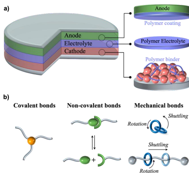
Figure 1 a) Typical “sandwich” structure of batteries, with potential polymeric components indicated. b) Schematic of conventional covalent bonds, non-covalent bonds and mechanical bonds (such as catenanes and rotaxanes) in polymer materials.
