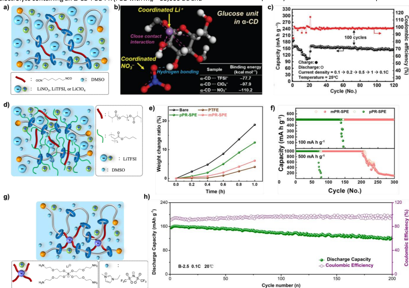
Figure 9 a) SRG electrolytes containing different salts. b) Interaction of \alpha -CD unit with \text{Li}^+ cation and salt anions in the SRG electrolytes. c) Performance of a full LFP||Li battery using a SRG electrolyte. d) SRG electrolyte comprising of copolymerized poly( n -butyl acrylate) and PEO diacrylate macrolinker through acrylate-functionalized \alpha -CD (mPR-SPE). e) the weight change of a bare Li metal, and ones coated with PTFE, SRG electrolyte containing unmodified CD (pPR-SPE) or mPR-SPE. f) Comparison of a Li|| \text{O}_2 full battery performance using pPR-SPE and mPR-SPE. g) SRG electrolyte crosslinked using a single-ion tetra-arm linker, and h) its performance in an NMC622||Li full battery. b) and c) are reproduced from reference [70] with permission from Wiley, copyright 2021, e) and f) are reproduced from reference [71], and f) is reproduced from reference [73] with permission from Wiley, copyright 2021.
