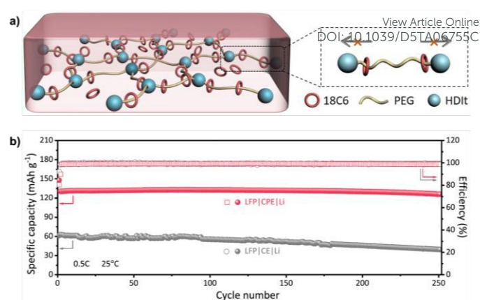
Figure 7 a) Schematic of a chain-end crosslinked PR network electrolyte (CPE) containing interlocked crown ethers, and b) its use in a LFP||Li full battery showing a stable and improved cycling at 25^\circ\text{C} , compared with a non-interlocked counter part CE. Reproduced from reference [64] with permission from American Chemical Society, copyright 2023.
