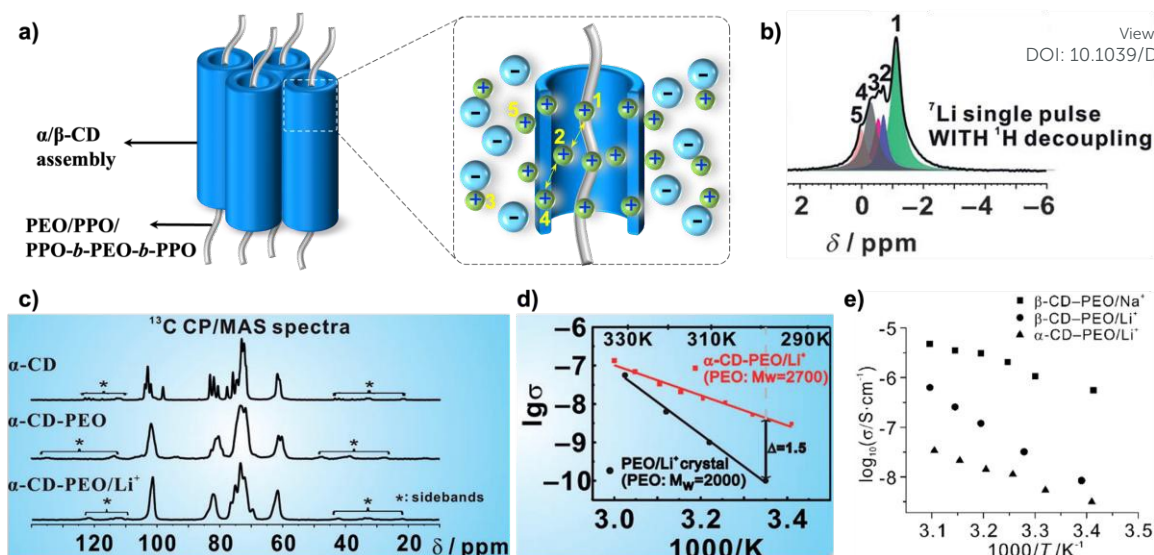
Figure 3 a) Pseudo-PR electrolytes consisting of nanochannels that enhance ion transport. b) Solid-state ^7\text{Li} NMR revealing five types of \text{Li}^+ species within the pseudo-PR electrolytes. c) ^{13}\text{C} CP/MAS spectra comparison of \alpha\text{-CD} , \alpha\text{-CD-PEO} and \alpha\text{-CD-PEO/Li}^+ , indicating the formation of nanochannels within the pseudo-PR electrolyte. d) Temperature-dependent ionic conductivity of pseudo-PR electrolyte and conventional PEO/Li electrolyte, demonstrating enhanced ion transport and distinct transportation mechanisms. e) Effect of host size and ion species on the ionic conductivity of pseudo-PR electrolytes containing nanochannels, where large host size enhances chain segmental motion and presumably lower charge density in ion species facilitates the ion transport within the nanochannels. b), c) and d) are reproduced from reference [45] with permission from Wiley, copyright 2014; e) is reproduced from reference [46] with permission from Wiley, copyright 2015.
