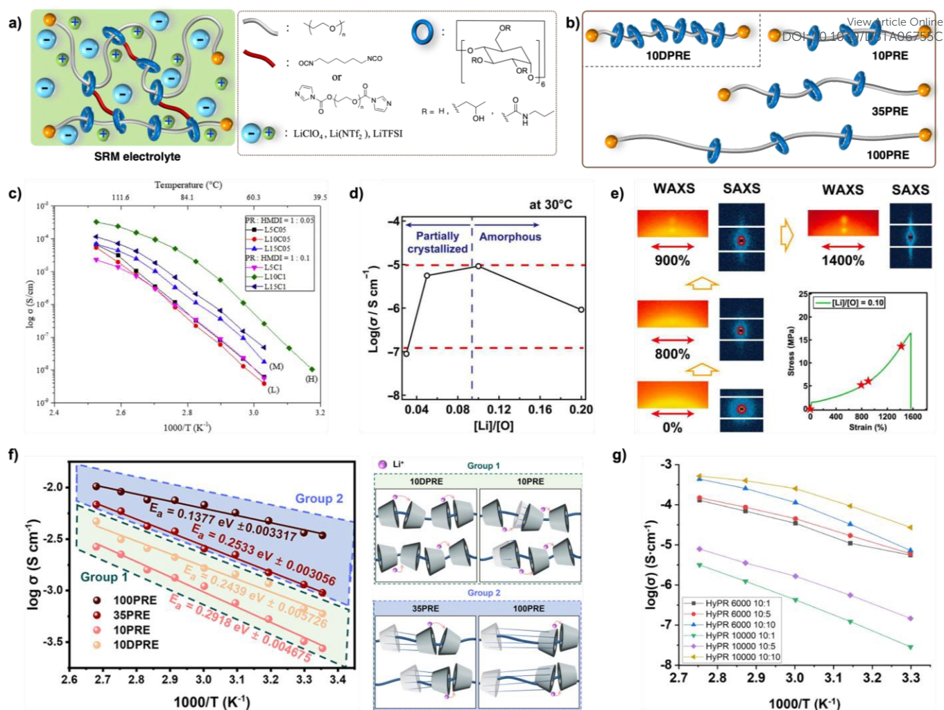
Figure 4 a) Compositions of SRM electrolytes in reported literature, with various crosslinkers, salts and modified CDs. b) Tunable PRs with varied axle lengths (10, 35 or 100 kDa) and wheel density (20 or 35 CDs per chian) for the fabrication of SRM electrolytes. c) Temperature-dependent ionic conductivity of SRM electrolyte with various salt contents and crosslinking densities. LxCy: x = 5, 10, 15 wt% Li(NTf 2 ) salt; y = 05 or 1 for 5 and 10 mol% hexamethylene diisocyanate crosslinker, respectively. d) Evolution of ionic conductivity over Li + /EO (or [Li]/[O]) ratio in the SRM electrolytes. e) WAX and SAXS studies of crystallinity in SRM electrolyte under different strains. f) Impact of PEO chain length and CD density in PR on the ionic conductivity of fabricated SRM electrolytes. g) Effects of the chain length of macrolinker and crosslinking density on the ionic conductivity of SRM electrolytes. For the legends, HyPR6000/10000 refers to the use of hydroxypropyl modified CDs and 6/10 kDa macrolinker, and the following ratio indicates the PR and macrocrosslinker weight ratios. c) is reproduced from reference [23] with permission from Elsevier, copyright 2018; d) and e) are reproduced from reference [49] with permission from Science Advanced, copyright 2024; f) reproduced from reference [50] with permission from American Chemical Society, copyright 2024; and g) reproduced from reference [51] with permission from American Chemical Society, copyright 2024.
