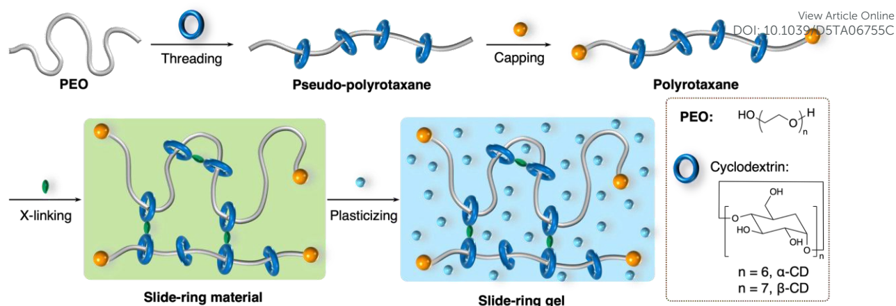
Figure 2 Representative scheme of preparation of mechanically interlocked polymer electrolytes using PEO and CDs. The materials generated in each step—pseudo-polyrotaxane (pseudo-PR), polyrotaxane (PR), slide-ring material (SRM) and slide-ring gel (SRG)—can be adapted to polymer electrolytes by introducing various salts.
