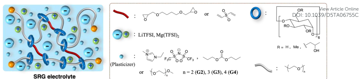
Figure 5 Schematic compositions of SRG electrolytes in reported literature, including various crosslinkers, salts, modified CDs and plasticizers.
