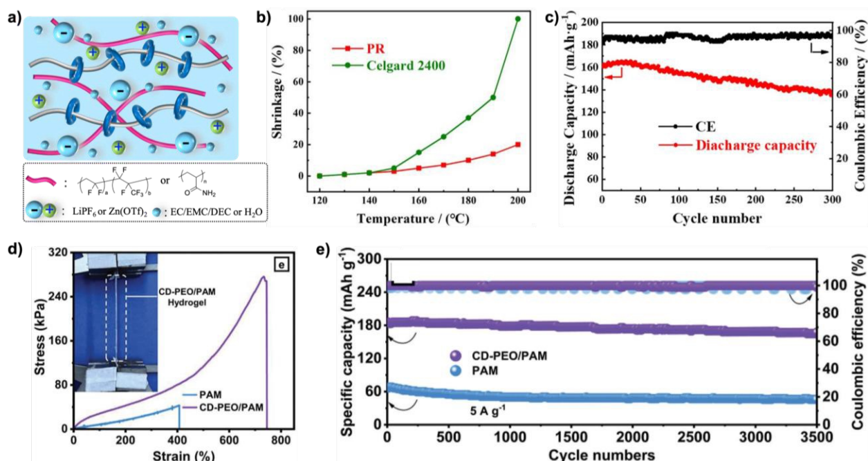
Figure 8 a) Composite gel electrolyte consisting of pseudo-PR and PVDF-HFP or PAM. b) Pseudo-PR composite gel electrolyte exhibits higher thermal stability than commercial Celgard 2400 membrane, and c) its use in a \text{NMC532}\|\text{Li} battery enables 86% capacity retention after 300 cycles at 0.5\text{C} . A CD-PEO/PAM composite electrolyte showed higher d) mechanical toughness and e) cycling capacity in a \text{La-V}_2\text{O}_5\|\text{Zn} battery than the PAM gel electrolyte. b) and c) are reproduced from reference [68] with permission from Springer, copyright 2022. d) and e) are reproduced from reference [69] with permission from Wiley, copyright 2023.
