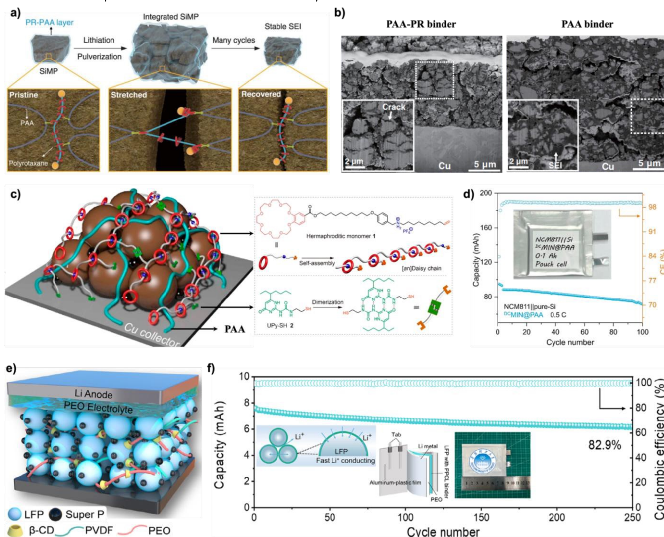
Figure 10 a) Mitigation of pulverization in the Si micro-particle (SiMP) anode during the battery cycling through the use of mechanically adaptive PR-PAA binder. b) Cross-sectional SEM images of SiMP anode after cycling using PR-PAA and PAA binders (after the 10 th delithiation. Si loading, 0.70 mg·cm -2 ; 0.2 C rate. c) Schematic of Si anode material fabricated using a novel MIP binder consisting of supramolecular crosslinked [an]daisy chains, and d) the cycling performance of a fabricated 100 mAh pouch cell. e) Illustrated full battery containing hybrid PVDF-PR electrode binder, and f) corresponding cycling performance of a fabricated pouch cell. The hybrid binder was indicated to facilitate the Li + transport at the electrode-electrolyte interface. a) and b) are reproduced from reference [27], c) and d) are reproduced from reference [79] with permission from American Chemical Society, copyright 2024, and e) and f) are reproduced from reference [80] with permission from Wiley, copyright 2025.
