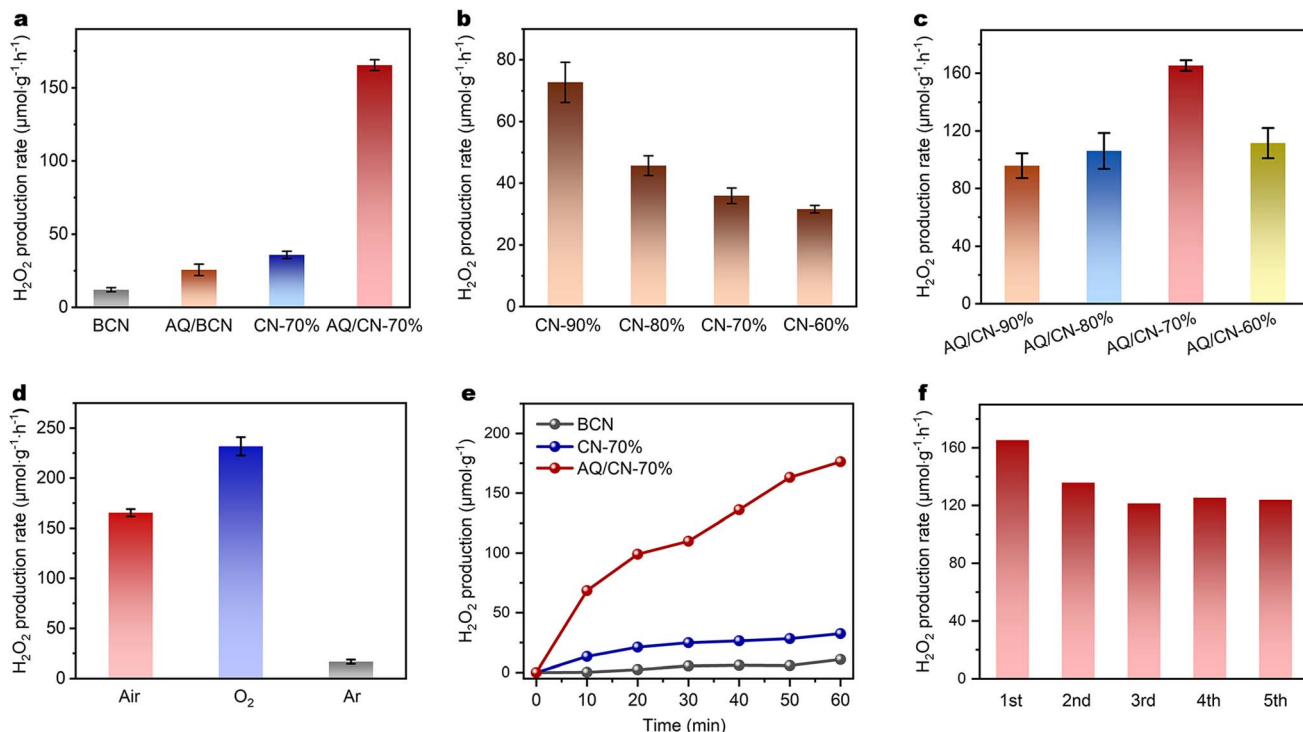
Fig. 2 (a) Photocatalytic H 2 O 2 production rates of BCN, AQ/BCN, CN-70% and AQ/CN-70%, (b and c) H 2 O 2 production rates of CN- x % and AQ/CN- x %, (d) photocatalytic H 2 O 2 production rate of AQ/CN-70% under varying atmospheres, (e) time-dependent H 2 O 2 production kinetics of BCN, CN-70% and AQ/CN-70%, and (f) photocatalytic cycling stability of AQ/CN-70% for H 2 O 2 production. Reaction conditions: 300 W Xenon light source equipped with a cut-off filter ( \lambda \geq 420 nm); irradiation intensity: 300 mW cm -2 ; reaction temperature: 25 °C.
