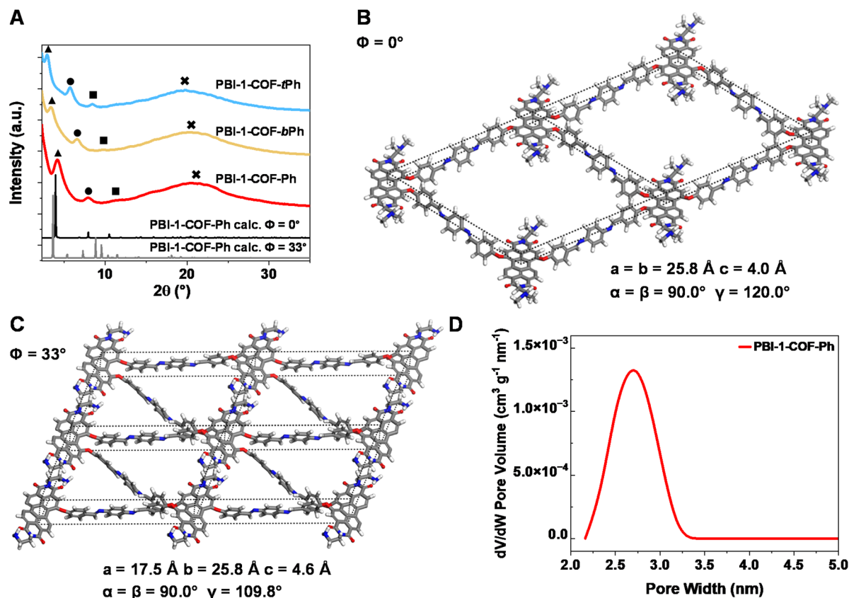
Fig. 3 (A) Experimental PXRD patterns of PBI-1-COF-Ph (red trace), PBI-1-COF- b Ph (yellow trace), and PBI-1-COF- t Ph (blue trace) along with the calculated PXRD patterns (black trace, \phi = 0^{\circ} ; grey trace, \phi = 33^{\circ} ) obtained by modelling an AA layer stacking mode for PBI-1-COF-Ph. (B) PBI-1-COF-Ph hexagonal unit cell and related parameters with \phi = 0^{\circ} . (C) PBI-1-COF-Ph triclinic unit cell and related parameters with \phi = 33^{\circ} . Both models were built and optimized using the Accelrys Material Studio 7.0 software package. (D) Pore size distribution of PBI-1-COF-Ph obtained from \text{N}_2 gas-volumetric measurements (DFT pore size method).
