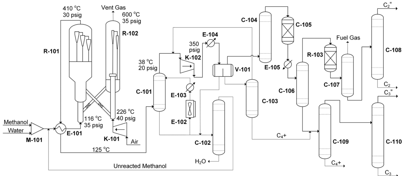
Fig. 7 Process flow diagram of MTO process adapted from UOP Co. 74 Unit identification: M-101 mixer; E-101 heat exchanger; R-101 fluidized reactor; R-102 regenerator; K-101 air compressor; C-101 quench tower; E-102 air-cooled exchanger; C-102 water stripper; K-102 product compressor; V-101 phase separator; C-103 condensate stripper; C-104 caustic scrubber; C-105 gas dryers; C-106 De-ethanizer; R-103 acetylene converter; C-107 De-methanizer; C-108 C_2 splitter; C-109 De-propanizer; C-110 C_3 splitter.
