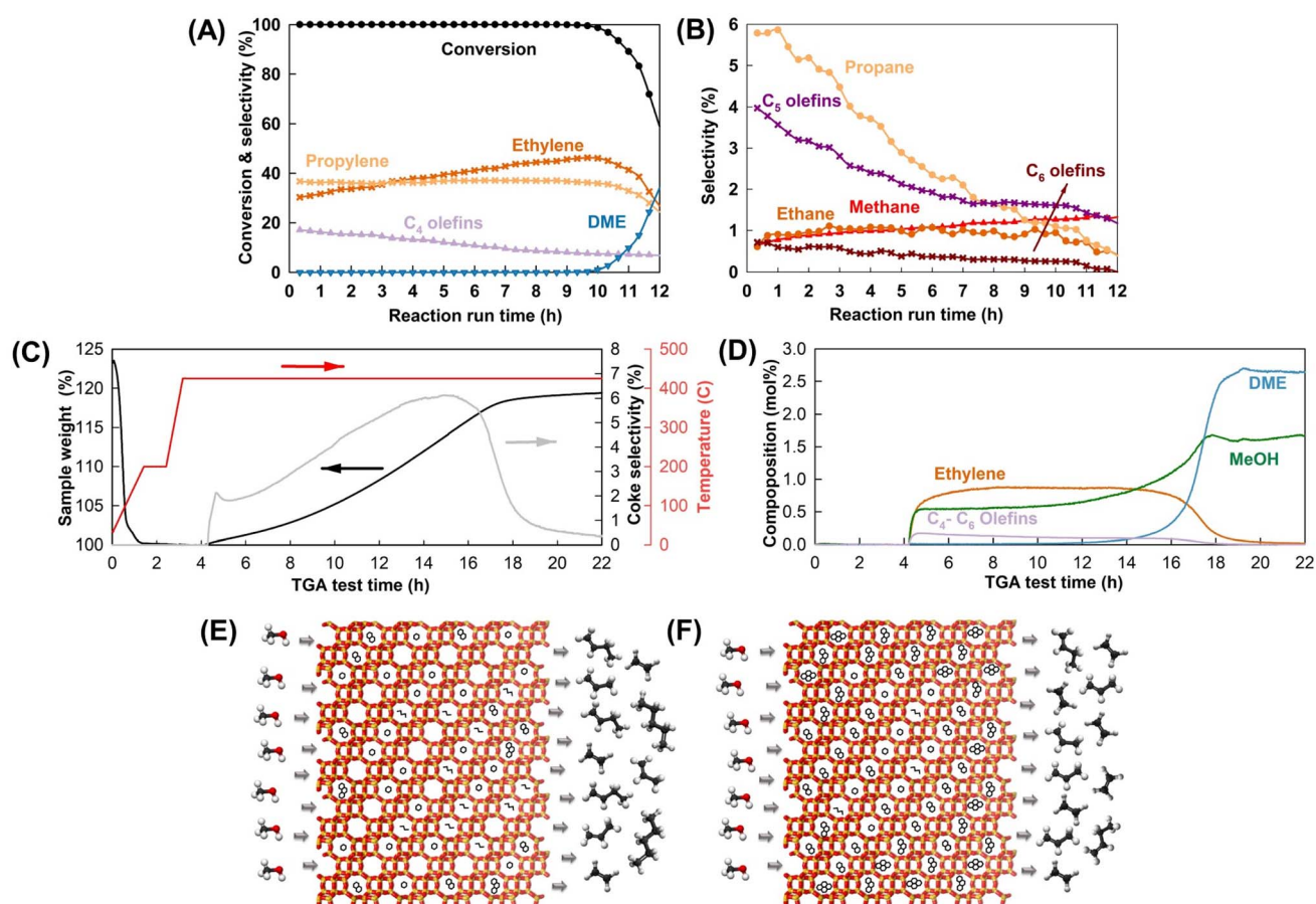
Fig. 8 (A and B) Products distribution versus time on stream over SAPO-34 catalyst in the MTO reaction. Reaction conditions: temperature of 400 °C, atmospheric pressure, WHSV of 1 \text{ g}_{\text{MeOH}} \text{ g}_{\text{Cat}}^{-1} \text{ h}^{-1} , and methanol diluted with 20 wt% water. (C and D) TGA-MS analysis: coke formation measurement using TGA and products distribution acquisition by MS. Reaction conditions: temperature of 400 °C, atmospheric pressure, WHSV of 1 \text{ g}_{\text{MeOH}} \text{ g}_{\text{Cat}}^{-1} \text{ h}^{-1} , and methanol diluted with 93 mol% argon. (E and F) Coke evolution in the pores of the SAPO-34 catalyst in (E) the beginning of the activity run, and (F) in enhanced times on stream close to catalyst deactivation. Reproduced from ref. 76 with permission from American Chemical Society, Copyright 2023.
