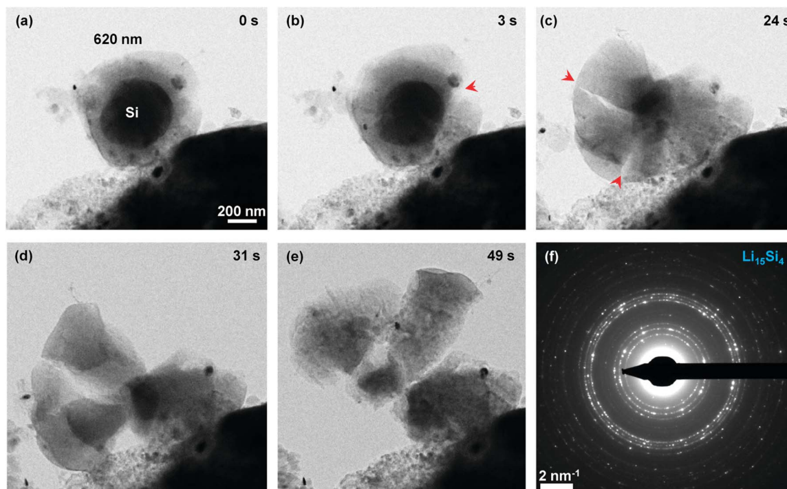
Fig. 2 (a–e) Lithiation of a 620 nm crystalline silicon particle with decrepitation. Red arrows indicate cracks. (f) Electron diffraction indicating the formation of polycrystalline \text{Li}_{15}\text{Si}_4 upon lithiation. Images reproduced from ref. 10.
