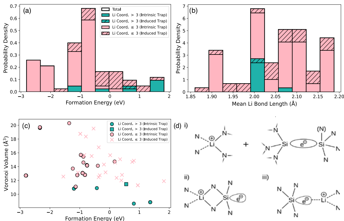
Fig. 2 (a) Distribution of Li-formation energies in \alpha - \text{Si}_3\text{N}_4 . The total distribution (black outline) is subdivided based on coordination (pink and turquoise) and trapping site (crosshatched). (b) Li-bond length distribution in the first coordination shell, with the same subdivision as in (a). Histogram bars represent the probability-density estimate p(x) = \frac{n_i}{N\Delta x} ; the distribution is normalised by \int p(x)dx = 1 . (c) Relationship between the Voronoi volumes of the incorporated Li atoms and the formation energies. (d) Schematic representation of the main Li-incorporation configurations in the \alpha - \text{Si}_3\text{N}_4 network.
