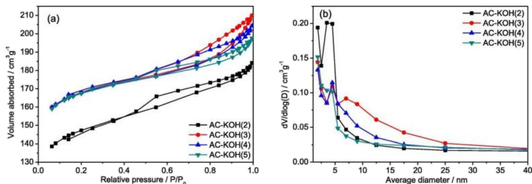
Fig. 13 \text{N}_2 adsorption and desorption isotherms 115 (a) of the activated carbon samples and the corresponding pore size distribution (b) calculated by the BJH method using the desorption branch of the isotherms.
