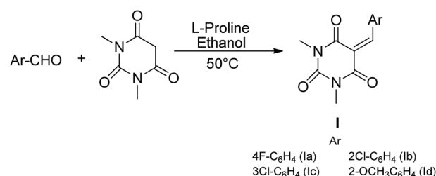
Scheme 1 Synthesis of benzylidene-1,3-dimethylpyrimidine-2,4,6(1 H ,3 H ,5 H )-triones.
