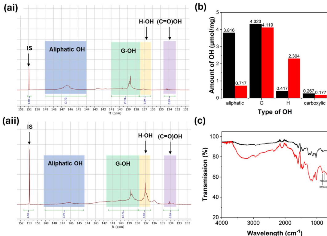
Fig. 10 (a) Liquid-state ^{31}\text{P} NMR collected of phosphitylated (i) KL and (ii) and KL-Ph. (b) Graph summarising the amounts of each different OH group present in KL before (black) and after (red) phenolation. (c) FTIR spectra of KL (black) and KL-Ph (red).
