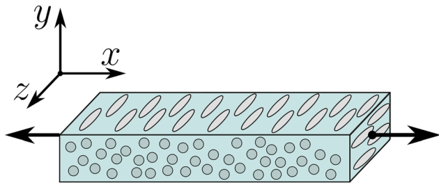
Fig. 2 Geometry and alignment of LCEs in this study. The nematic director in the unstrained LCEs is along the z-axis, strain is applied along the x-axis. The thickness of the LCE, i.e. the dimension in which the auxetic response is observed, is along the y-axis.
