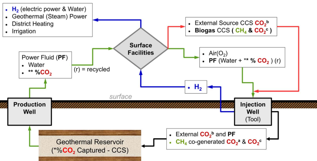
Fig. 3 A flow diagram of the CLGG wellbore reformation process. \text{CO}_2^{\text{a}} = \text{CO}_2 generated by reformation of methane, \text{CO}_2^{\text{b}} = \text{CO}_2 obtained from external industry sources, \text{CO}_2^{\text{c}} = the natural \text{CO}_2 content held within biogas, \% \text{CO}_2 = the % of the injected \text{CO}_2 that is retained within the reservoir, \% \text{CO}_2^{\text{**}} = the % of the injected \text{CO}_2 that is recirculated within the power fluid, CCS = Carbon Capture and Storage.
