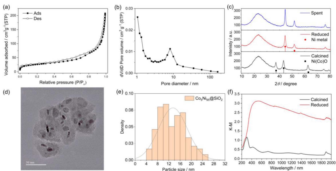
Fig. 2 Characterization results of the Co 5 Ni 95 @SiO 2 catalyst. (a) N 2 adsorption–desorption isotherm. (b) Pore size distribution of the calcined sample. (c) XRD patterns of the calcined, reduced and spent catalysts. (d and e) TEM image and particle size distribution of the reduced catalyst. The scale bar is 50 nm. (f) UV-visible DRS of the calcined and reduced catalysts.
