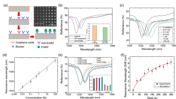
Fig. 1 (a) Schematic of the label-free assay and SEM of the SNPs. (b) Reflection spectra of the bare sensor, GO layer, and anti- ErbB2 antibody coating. (c) Reflection spectra in the presence of ErbB2 . (d) Dose-response curve for the detection of ErbB2 . (e) Reflection spectra for seven different combinations of ErbB2 , ErbB3 , and ErbB4 antigens. Inset: resonance wavelength in presence of antigens and interfering molecules. (f) Simulation and experimental results for the binding of ErbB2 and anti- ErbB2 antibodies. Reproduced from ref. 26 with permission from Elsevier, copyright 2018.
