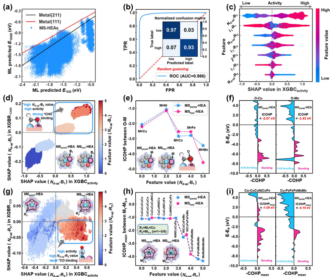
Fig. 2 (a) ML-predicted \Delta E_{\text{CO}} and \Delta E_{\text{CHO}} values for all MS-HEAs. The solid lines denote the scaling relations on metal (211) substrate (black) and metal (111) substrate (red). (b) ROC curve and normalized confusion matrix of XGBC activity . (c) SHAP summary plots of every feature in XGBC activity . The bidirectional arrows at the top of the figure show the relationship between the SHAP values and activity. (d) The relationship between the feature value of N_{\text{d-up}}-B_1 and SHAP values of N_{\text{d-up}}-B_1 in XGBC activity and XGBC activity . (e) ICOHP and (f) COHP between the O atoms of *CHO and metal atoms in the B_1 region (with different values of N_{\text{d-up}}-B_1 ). (g) The relationship between the feature value of N_{\text{d-up}}-R_2 and SHAP values of N_{\text{d-up}}-R_2 in XGBC activity and XGBC activity . The (h) mean ICOHP and (i) COHP between the Cu atoms in the R_1 region and metal atoms in the R_2 region (with different values of N_{\text{d-up}}-R_2 ).
