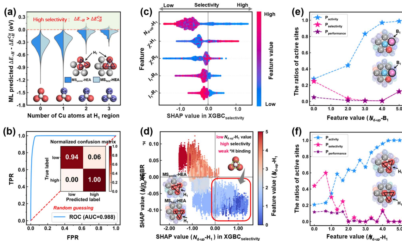
Fig. 3 (a) Distributions of the difference between the ML-predicted \Delta E_{\text{H}} values of all MS-HEAs and \Delta E_{\text{H}} values on a pure Cu 55 cluster. (b) Receiver operating characteristic (ROC) curve and normalized confusion matrix of XGBC selectivity for model evaluation. (c) SHAP summary plots of every feature in XGBC selectivity . The color of each dot represents the feature value. The bidirectional arrows at the top of the figure show the relationship between the SHAP values and selectivity. (d) The relationship between the feature value of N_{\text{d-up}}\text{-H}_1 and SHAP values of N_{\text{d-up}}\text{-H}_1 in XGBC activity and XGBC selectivity . The ratios of active sites ( P_{\text{activity}} , P_{\text{selectivity}} , and P_{\text{performance}} ) in FeCoNiCuMo MS-HEAs with various key feature values of (e) N_{\text{d-up}}\text{-B}_1 or (f) N_{\text{d-up}}\text{-H}_1 .
