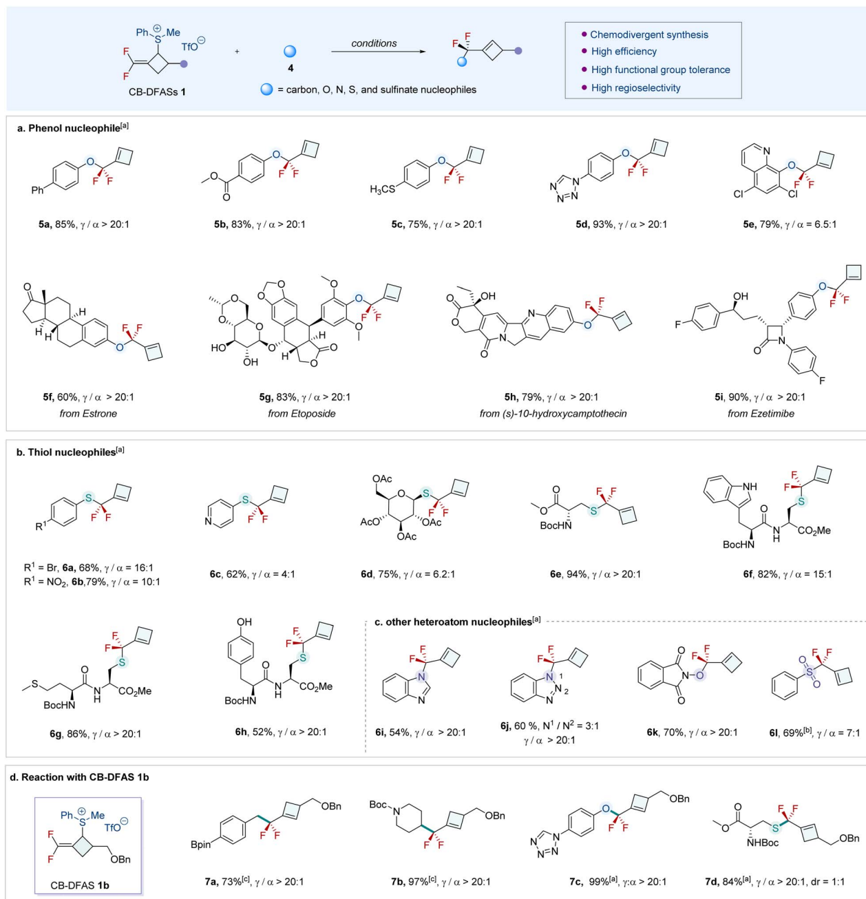
Scheme 4 Reaction of nucleophiles with CB-DFASs 1. [a] Conditions A: 1a (1.2 equiv.), heteroatom nucleophile 4 (0.2–0.3 mmol 1.0 equiv.), \text{K}_2\text{CO}_3 (2.0 equiv.), acetone (2.0 mL), rt, 3 h; [b] condition B: 1a (0.2 mmol, 1.0 equiv.), sodium benzenesulfinate (1.2 equiv.), \text{K}_2\text{CO}_3 (0.4 mmol, 2.0 equiv.), DMSO (2.0 mL); [c] conditions C: 1b (1.05 equiv.), 2 (0.2 mmol 1.0 equiv.), CuBr (5 mol%), THF (2.0 mL), rt, 3 h. All reported yields are isolated yields.
