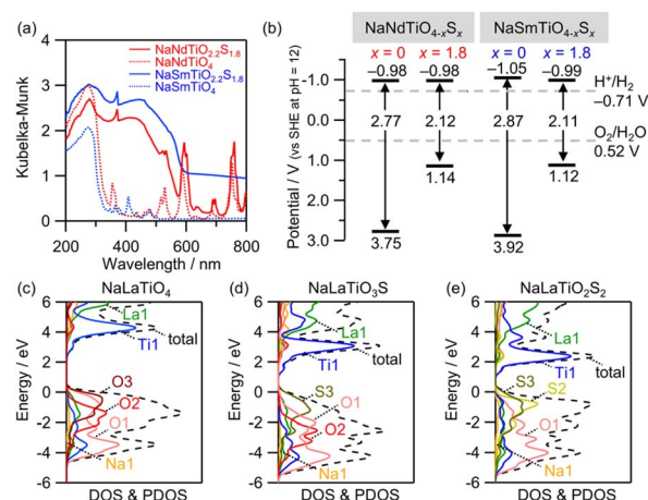
Fig. 7 (a) UV-vis diffuse reflectance spectra and (b) band edge positions at \text{pH} = 12 of \text{NaMTiO}_4 and \text{NaMTiO}_{2.2}\text{S}_{1.8} ( M = \text{Nd}, \text{Sm} ). DOS and PDOS near the VBM and CBM of (c) \text{NaLaTiO}_4 , (d) \text{NaLaTiO}_3\text{S} , and (e) \text{NaLaTiO}_2\text{S}_2 calculated using the structural models shown in Fig. S18.
