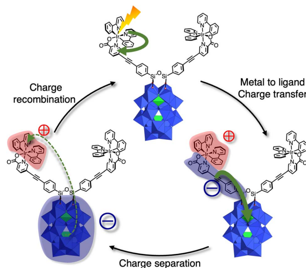
Fig. 5 Directionality in the photoinduced electron transfers of the POM-Ir(III) assembly [P_2W_{17}O_{61}\{O(SiC_3H_6O_2)_2N_3Ir\}_2]^{6-} , conferred by the heteroleptic character of the Ir(III) complex. The red and blue cloud respectively represent the localization of the positive and negative charges in the different excited states. 51
