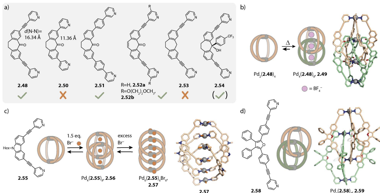
Fig. 9 Interlocked double cages \text{Pd}_4\text{L}_8 . (a) Structures of suberone-based ligands 2.48 – 2.54 (check mark: forms a double cage; cross: does not form a double cage). (b) Self-assembly of monomeric cage \text{Pd}_2(\text{2.48a})_4 as a kinetic product and double cage 2.49a as the thermodynamic product. (c) Halide induced formation of double cage 2.56 and ligand release upon addition of excess halides to form triple catenated 2.57 in the solid state. (d) Triply interlocked double cage 2.59 with furane based ligand 2.58 .
