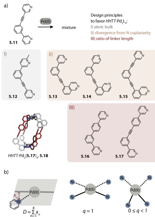
Fig. 22 (a) Modification of ligand \mathbf{5.11} by using (I) steric bulk on the donor site, (II) alteration of the offset between the nitrogen donor groups, and (III) increase in the difference in the linker lengths for steering orientational self-sorting to the HHTT - \text{Pd}_2\text{L}_4 isomer and crystal structure of HHTT - \mathbf{5.18} . (b) Illustration of heuristics D , the maximal sum of the deviations of the Pd(II)-nitrogen bonds from the average \text{PdN}_4 plane and q , the minimum square planar order parameter for estimating the stability of cage isomers.
