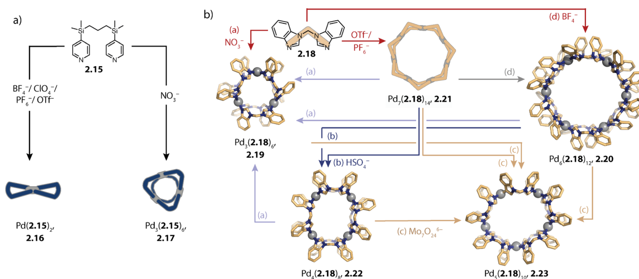
Fig. 5 Self-assembly of homoleptic rings \text{Pd}_n\text{L}_n ( n = 3-7 ) by templation. (a) Flexible ligand 2.15 self-assembles to form entropically favoured lemniscate 2.16 or via templation to the three-membered ring 2.17 . (b) Flexible, small ligand 2.18 assembles to form rings 2.19 – 2.23 of various sizes depending on the counter anion(s) present.
