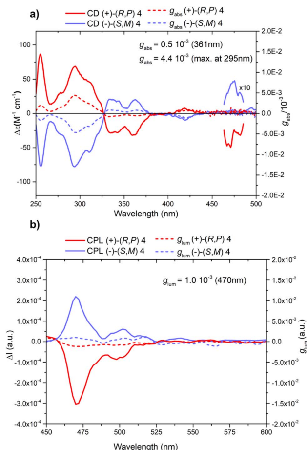
Fig. 5 (a) Circular dichroism absorption spectra (solid lines) for both enantiomers (+)-4 (in red) and (–)-4 (in blue) (CHCl 3 , 20 °C, 6 μM) and absorptive dissymmetry factor ( g_{\text{abs}} ) (dashed lines); (b) CPL spectra (solid lines) of (+)-4 (in red) and (–)-4 (in blue) and luminescence dissymmetry factor ( g_{\text{lum}} ) (dashed lines) ( \lambda_{\text{exc}} = 390 nm, CHCl 3 , 20 °C, ~1 μM).
