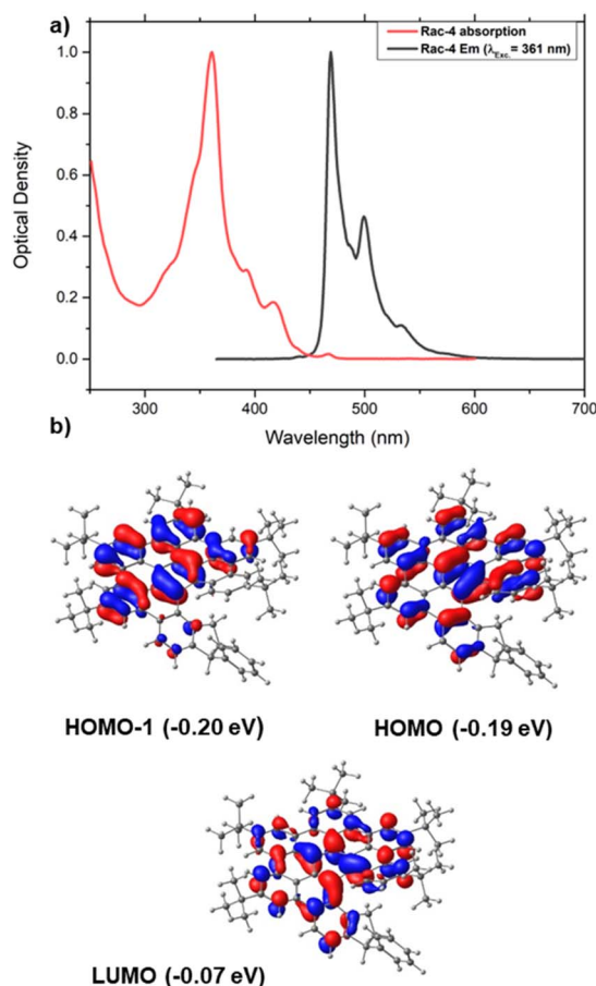
Fig. 4 (a) UV/vis absorption spectra of racemic 4 and normalized fluorescence emission spectra (black line) in CH 2 Cl 2 (1.8 μM) upon irradiation at the absorption maximum. (b) Computed molecular orbitals of (S,M)-4 involved in the lower energy absorptions (isosurface value of 0.03 a.u.).
