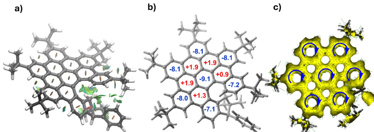
Fig. 3 (a) Contour plots of the reduced density gradient isosurfaces (density cutoff of 0.045 a.u.) for (S,M)-4. The green surfaces indicate attractive noncovalent interactions. (b) Computed NICS values (in ppm). (c) AlCD plot (isosurface value of 0.04 a.u.).
