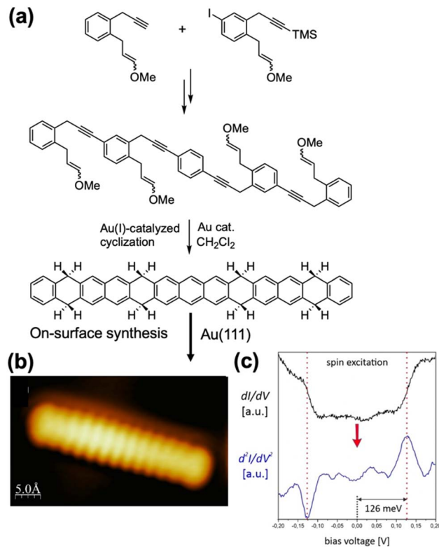
Fig. 13 (a) Synthesis of the tridecane precursor and (b) STM image of on-surface generated tridecane. (c) Single point STS spectra acquired over tridecane, exhibiting a symmetric step-like appearance (top) together with numerically differentiated d^2I/dV^2 spectra showing the presence of pronounced resonances centred at approximately \pm 126 meV. Adapted with permission from ref. 63. Copyright 2023 Wiley.
