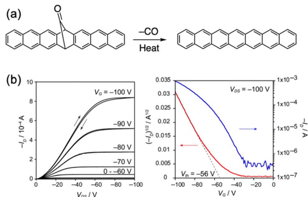
Fig. 31 (a) Heptacene generation from its monoketone precursor. (b) Output (left) and transfer characteristics (right, V_{DS} = -100 \text{ V} ) of heptacene thin films. Adapted with permission from ref. 114. Copyright 2021 Wiley.
