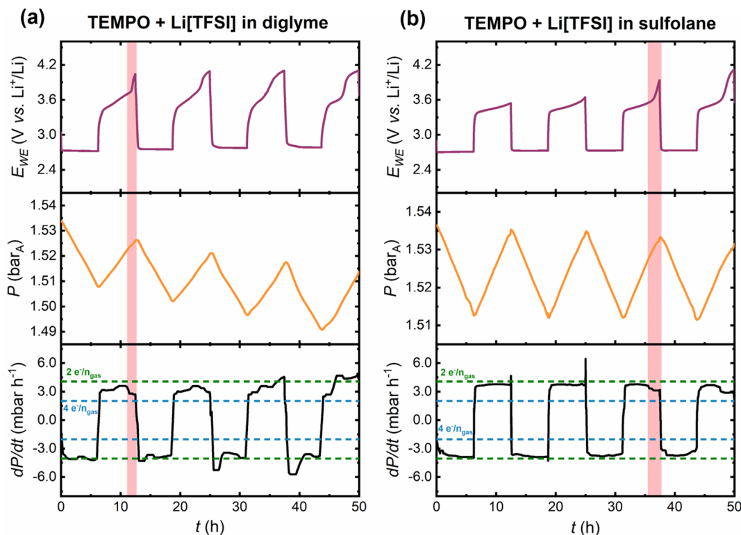
Fig. 5 Cycles 1–4 in the pressure cells cycled under a capacity-limited ( 500 \text{ mAh g}^{-1} ) regime at 80 \text{ mA g}^{-1} in TEMPO-mediated (a) diglyme- and (b) sulfolane-based electrolytes. The RM loading was 25 \text{ mmol}_{\text{TEMPO}} \text{ kg}_{\text{solvent}}^{-1} and the mole fraction ( x ) ratio of solvent : Li[TFSI] salt was x_{\text{solvent}} : x_{\text{Li[TFSI]}} = 9 : 1 . The cell potential (purple), pressure response (orange) and first derivative of the pressure response (black) are shown as a function of time. The dotted green and blue lines indicate the theoretical gas consumption/evolution rates for 2e^-/n_{\text{gas}} and 4e^-/n_{\text{gas}} processes, respectively. The red shaded regions highlight the sensitivity of the pressure measurement, capturing drops in gas evolution rate that coincide with sharp rises in cell potential, which serve as a marker for decreased RM efficacy.
