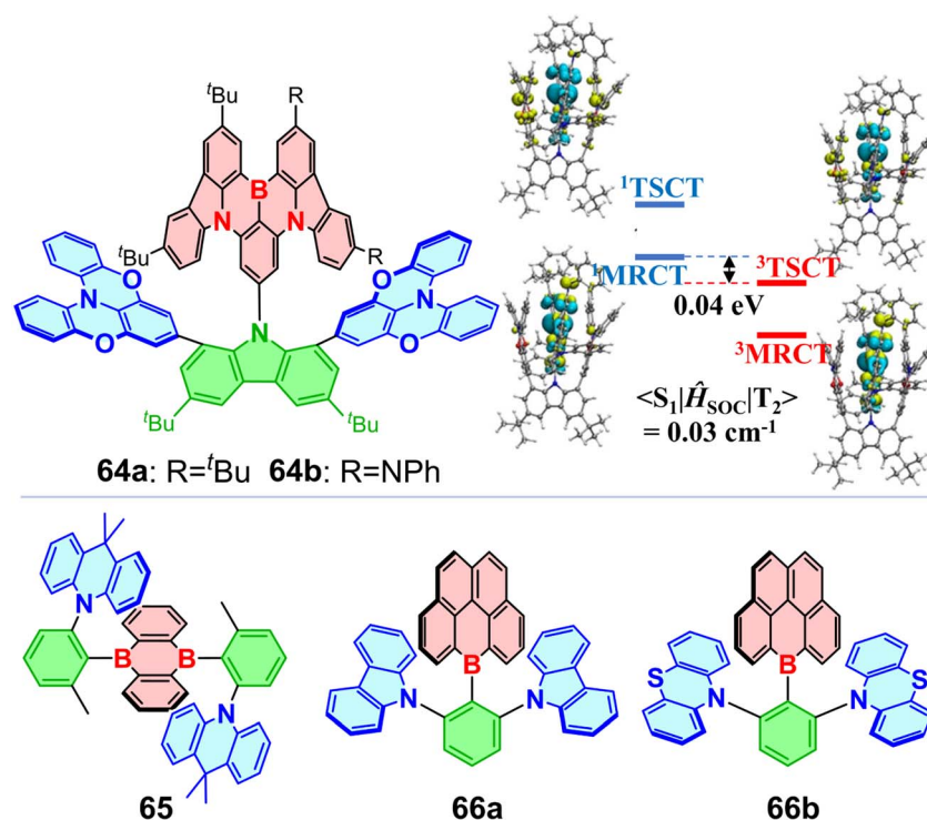
Fig. 20 TSCT OBCTs with different planar boron acceptors. The illustration showing calculated hole (green) and electron (blue) distributions and energy gaps of the ^1\text{MRCT} and ^1\text{TSCT} excited states for 64b . Copyright 2023, John Wiley & Sons.
