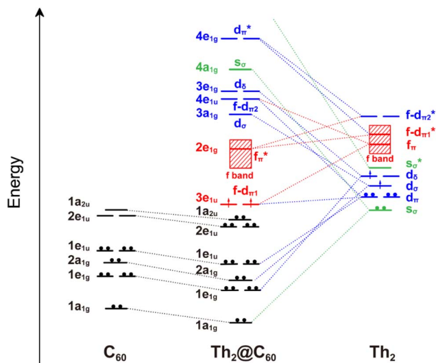
Fig. 4 Orbital interaction diagram for \text{Th}_2\text{C}_{60} molecules, illustrating the bonding scheme between neutral \text{C}_{60} and the \text{Th}_2 dimer. The arrows represent the unpaired single-electron bonds of the \text{Th}_2 dimer, and the dots represent the electron-pair bonds. The orbitals of the neutral \text{Th}_2 dimer are shown in Fig. S19.†
