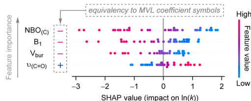
SHAP analysis in NN model
