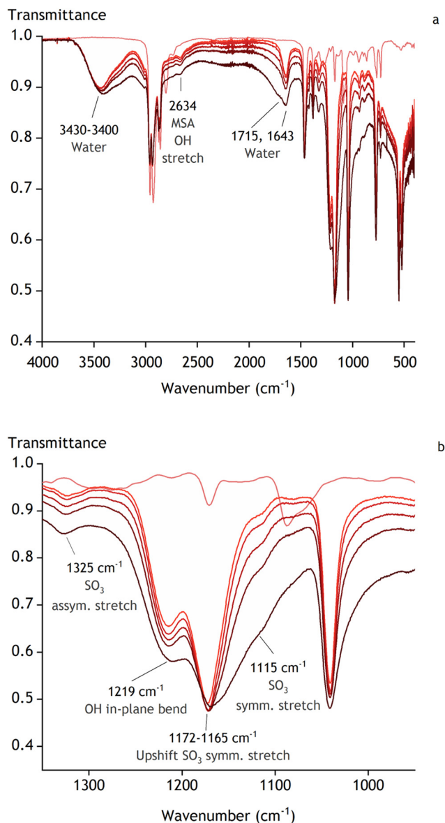
Fig. 5 FTIR spectra of TEHA loaded with increasing MSA concentrations from light red to black. 1% L and 0.003\text{ mol L}^{-1} H_2O (—), 95% L (—), 112% L and 4.2\text{ mol L}^{-1} H_2O (—), 122% L and 4.3\text{ mol L}^{-1} H_2O (—), 137% L and 5.3\text{ mol L}^{-1} H_2O (—), 179% L and 6.3\text{ mol L}^{-1} H_2O (—). (a) Shows the full spectra, while (b) displays a zoom on the most relevant region for MSA vibrations.
