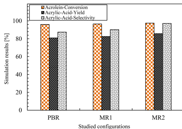
Fig. 15 Acrolein conversion, acrylic acid yield, and acrylic acid selectivity for three cases PBR, MR1, and MR2 (at temperature 583.5 K, \text{GHSV} 1600 \text{h}^{-1} , and oxygen/acrolein molar ratio of 5.7).
