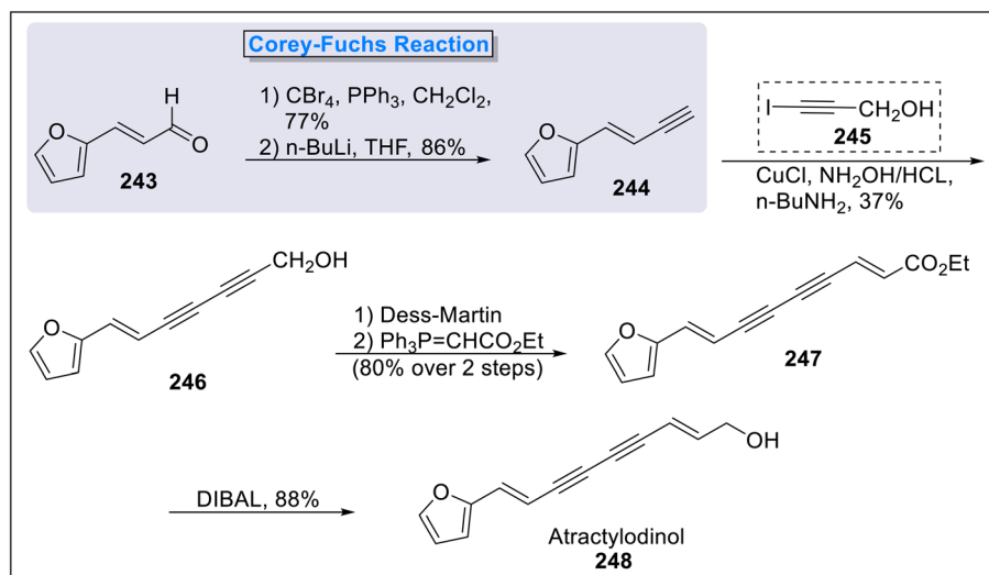
Scheme 24 Total synthesis of atractylodiol 248 by Kraus and coworkers.
