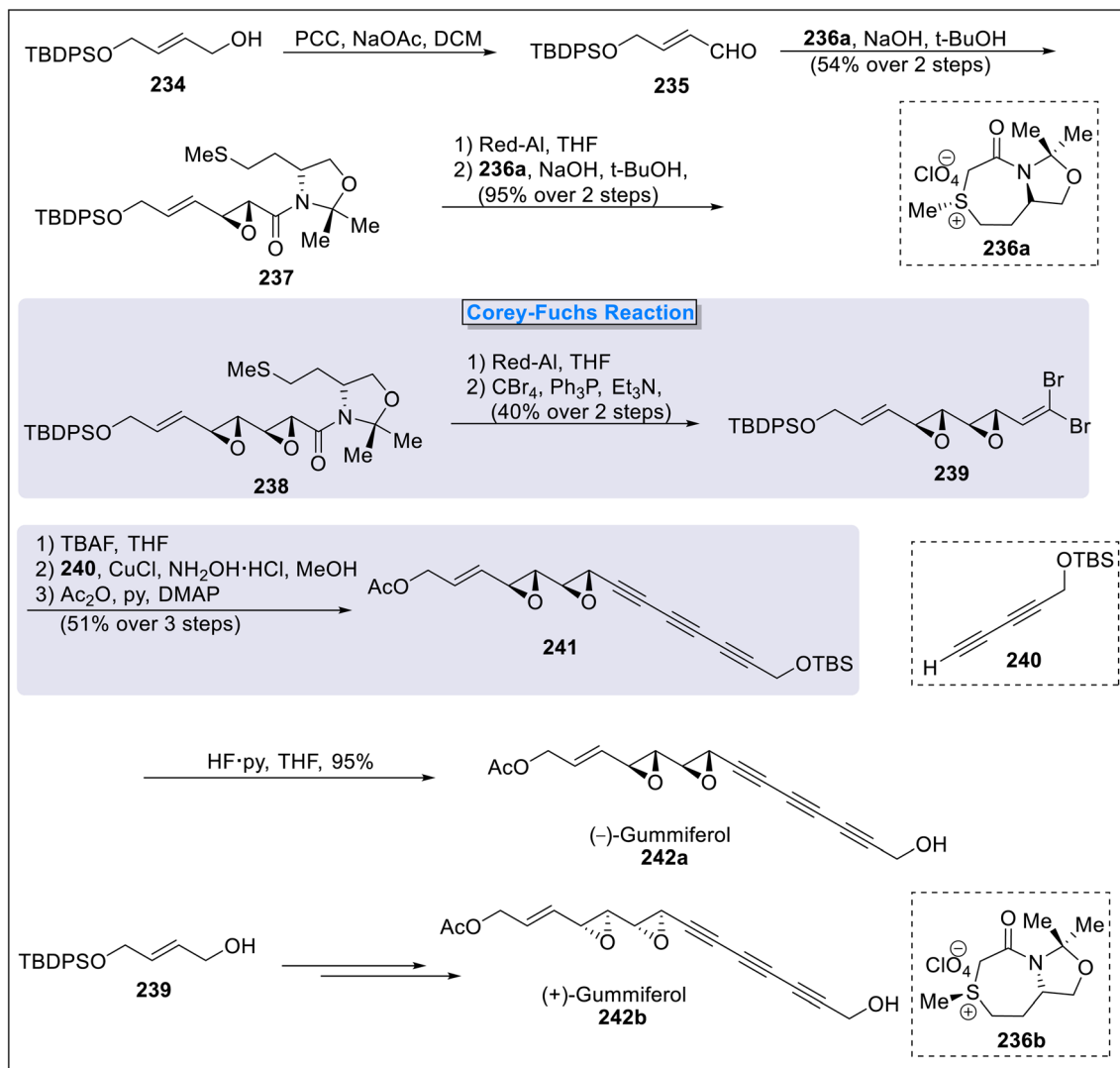
Scheme 23 Total synthesis of (-)-gummiferol 242a &amp; (+)-gummiferol 242b by Sarabia and coworkers.
