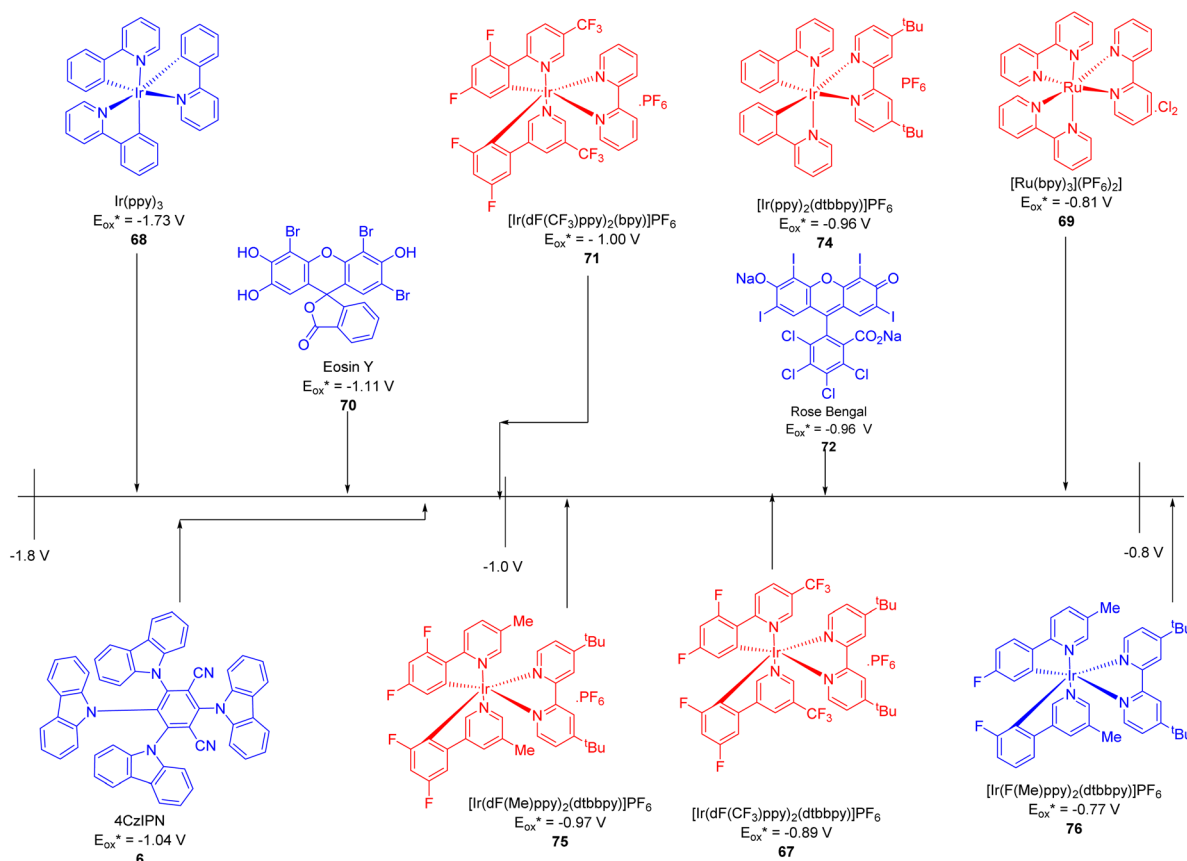
Fig. 49 E_{\text{ox}}^* of common visible light PCs. Reproduced from ref. 208, https://doi.org/10.1039/D1CS00198A , under the terms of the CC BY-NC 3.0 license, https://creativecommons.org/licenses/by-nc/3.0/ .
