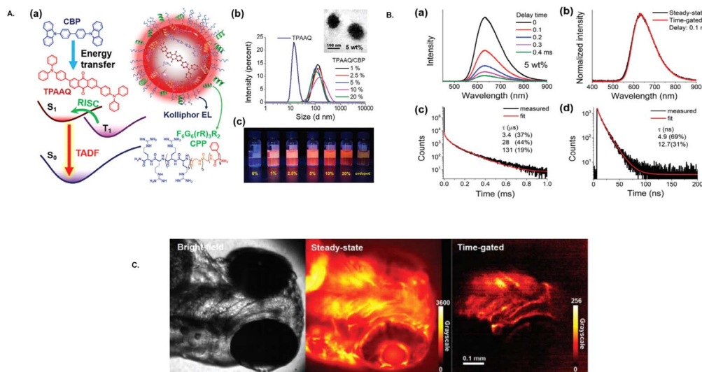
Fig. 24 (A) (a) Representation of TPAAQ/CBP/CPG TADF nanoparticles (b) DLS histograms showing the size of the nanoparticles and inset TEM images showing their morphology. (c) Photographs of the nanoparticle solutions under UV irradiation. (B) Time-gated emission spectra of the nanoparticles at various delay times. (C) Imaging of zebrafish incubated with TPAAQ/CBP/CPG nanoparticles, where the bright field is displayed on the left side of the figure, the steady-state luminescence is shown in the middle, and the time-gated luminescence is displayed on the right. Reproduced from ref. 173 with permission from John Wiley & Sons, Copyright © 2024, Wiley-VCH Verlag GmbH & Co. KGaA, Weinheim.
