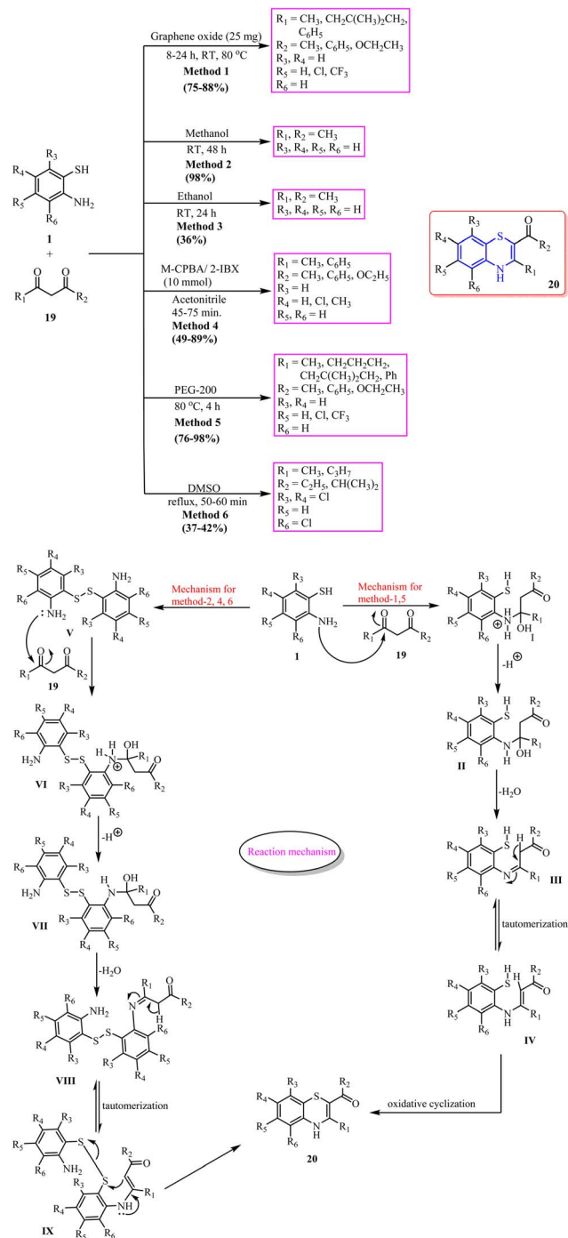
Scheme 7 Synthesis of 1,4-BT using 2-ATP and 1,3-dicarbonyls.
