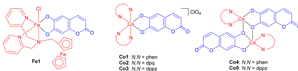
Fig. 10 Earth-abundant metal PSs with coumarin directly coordinated as O^N,O ligand.
