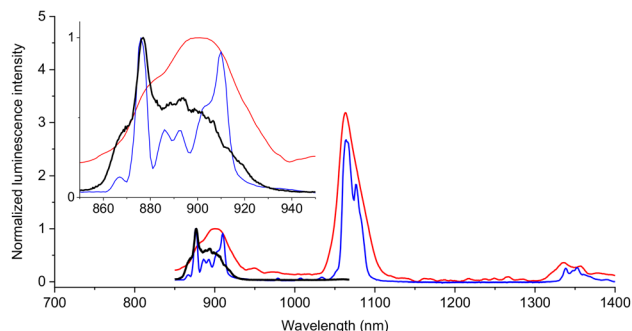
Fig. 3 Comparison of the normalized ECL (black line) and PL emission spectra of 1Ru-Nd at room temperature (red line, \lambda_{\text{exc}} = 450 \text{ nm} ) and at 77 K in frozen organic glass (blue line) with the same experimental conditions as in Fig. 2. The ECL spectra of 1Ru-Nd were recorded at an imposed potential of 1.9 V. The inset shows a zoomed-in view of the 850–950 nm area.
