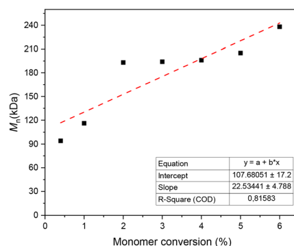
Fig. 1 Linear regression of M_n vs. monomer conversion determined by ^1\text{H} NMR spectroscopy at room temperature using 0.1 mol% ( \text{LaCl}_3/[\text{Cu}(\text{CH}_3\text{CN})_4]\text{PF}_6 ) as catalyst.
