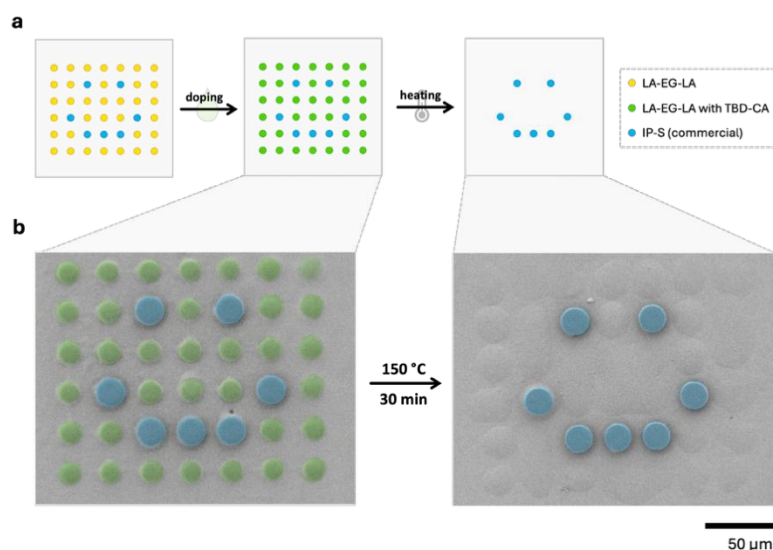
Fig. 6: a) Schematic representation of the multi-material printing process and the subsequent doping and depolymerisation of the 3D microprinted structures, b) SEM images of an array of pillars printed with IP-S and LA-EG-LA before and after heating to 150 ^{\circ}\text{C} , causing the pillars of LA-EG-LA doped with TBD-CA to depolymerise (subsequently coloured for visual distinction).
