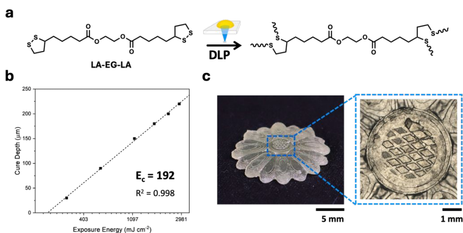
Fig. 2: a) Photopolymerisation reaction of LA-EG-LA for the formation of a polymer network during the DLP printing process. b) Jacobs working curves of LA-EG-LA with an LED at 405 nm. c) 3D printed flower printed with a layer thickness of 100 µm and a light intensity of 55 mW/cm 2 , light microscope image showing the highly detailed centre of the 3D printed flower.
