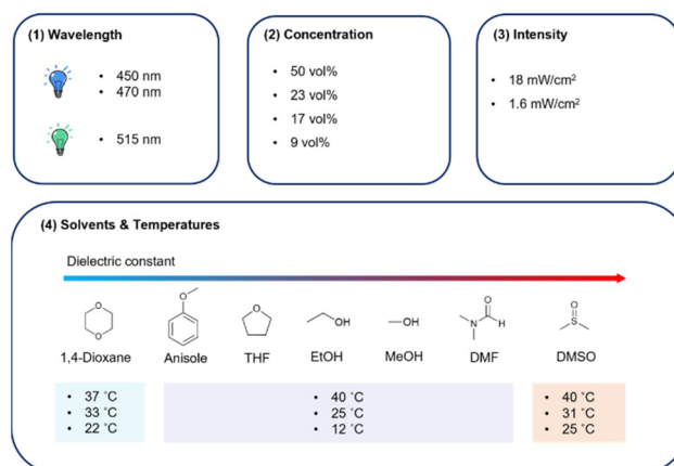
Fig. 1 P(PEGMA) synthesis scheme through the PI-RAFT approach and overview of this study. The synthesis in 1,4-dioxane and DMSO cannot be conducted at 12 °C because of the high melting point of solvents.
