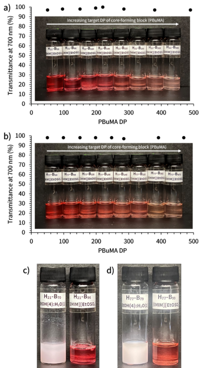
Fig. 3 Images showing the physical appearance of the series of (a) PHEMA 21 -b-PBuMA y and (b) PHEMA 77 -b-PBuMA y block copolymer dispersions in [EMIM][EtOSO 3 ] at 10% w/w solids alongside corresponding transmittance values obtained from UV-vis spectroscopy. Labels on sample vials denote the actual PHEMA x -b-PBuMA y composition, denoted as H x -B y , as determined using 1 H NMR spectroscopy. Images comparing the PHEMA 21 -b-PBuMA y (c) and PHEMA 77 -b-PBuMA y (d) prepared in an EtOH/H 2 O solvent mixture (left) and [EMIM][EtOSO 3 ] (right).
