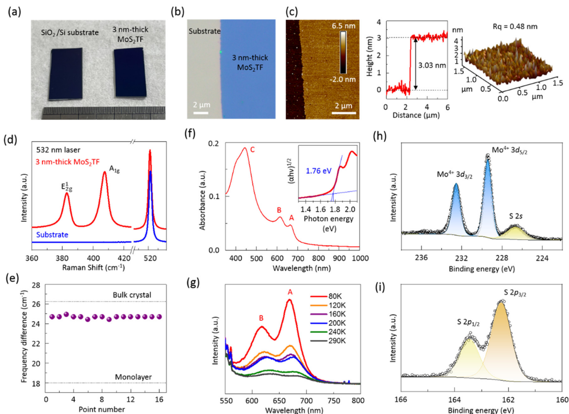
Fig. 2 (a) Photographs of the \text{SiO}_2/\text{Si} substrates before (left) and after (right) the growth of the 3 nm-thick \text{MoS}_2\text{TF} . (b) Optical microscopy image and (c) atomic force microscopy (AFM) images of the as-grown 3 nm-thick \text{MoS}_2\text{TF} , including surface height profiles and surface roughness characterization on the \text{SiO}_2/\text{Si} substrate. (d) Raman spectra of the 3 nm-thick \text{MoS}_2\text{TF} and the bare \text{SiO}_2/\text{Si} substrate, recorded using a 532 nm excitation laser. (e) Statistical distribution of the frequency difference between the \text{A}_{1g} and \text{E}_{2g}^1 Raman modes obtained from 16 different points on the 3 nm-thick \text{MoS}_2\text{TF} . Distributions from commercial monolayer and bulk \text{MoS}_2 crystals are included for comparison. (f) UV-vis-NIR absorption spectrum and (g) temperature-dependent photoluminescence (PL) spectra of the 3 nm-thick \text{MoS}_2\text{TF} . The inset in (f) shows the Tauc plot used to estimate the optical band gap. (h and i) High-resolution XPS spectra of the Mo 3d (h) and S 2p (i) core-level regions for the 3 nm-thick \text{MoS}_2\text{TF} on the \text{SiO}_2/\text{Si} substrate.
