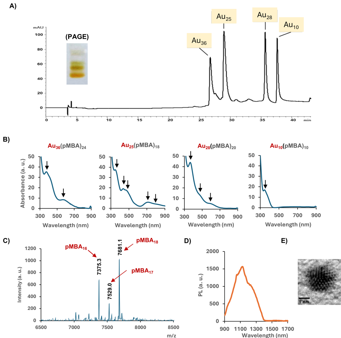
Fig. 1 (A) RP-HPLC analysis coupled with absorbance measurements for the Au 25 pMBA 18 crude reaction mixture, eluted on a gradient from 0% to 20% acetonitrile in 10 mM TEAA buffer, showing different AuNC subspecies eluted at different retention times; inset shows a photograph from PAGE analysis of the same Au(pMBA) crude reaction mixture. (B) Corresponding absorbance spectra of each eluted subspecies. (C) MALDI-ToF MS spectrum of purified Au 25 pMBA 18 . (D) NIR-II PL spectrum of Au 25 pMBA 18 dispersed in water; \lambda_{\text{exc.}} = 808 nm. (E) HRTEM image of Au 25 pMBA 18 .
