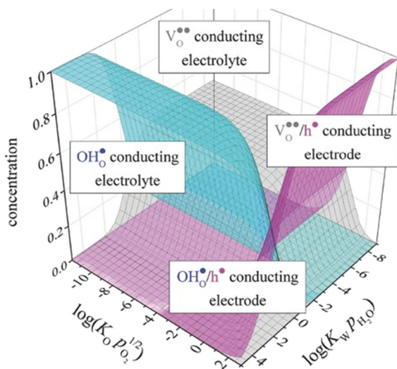
Fig. 7 The concentration of holes, oxygen ions and hydroxyl groups in perovskite oxides as a function of water partial pressure ( P_{H_2O} ) oxygen partial pressure ( P_{O_2} ) and equilibrium constants of hydration reaction ( K_W ) and oxygenation reaction ( K_O ). This figure has been adapted from ref. 122 with permission from John Wiley & Sons, copyright 2025.
