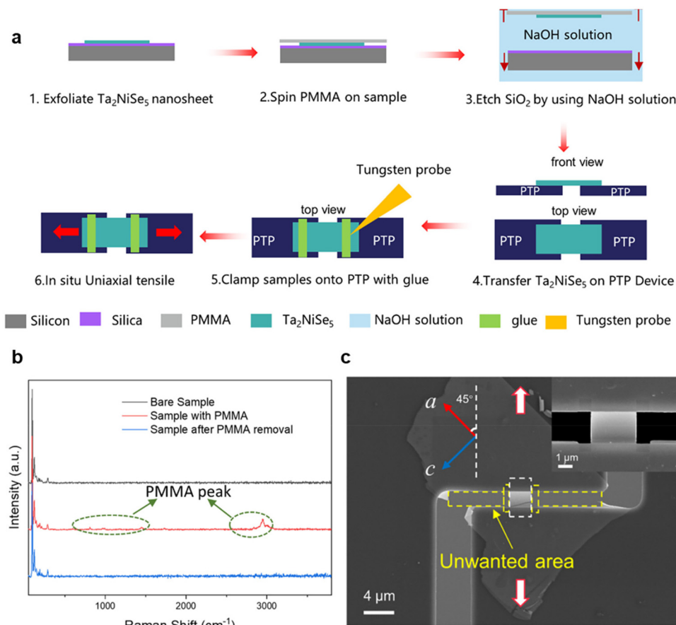
Fig. 6 A schematic showing the typical transfer process for 2D materials samples onto MEMS chips, composed of three steps. (a) The polymer-assisted transfer process onto MEMS chips. 28 (b) Removal of the polymer after transfer, confirmed by Raman spectroscopy. 28 (c) The clamping and shaping of sample under FIB. 28
